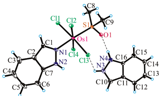
Figure 4. ORTEP view of 2 with atom labeling scheme; the thermal ellipsoids are shown at 50% probability level. Selected bond lengths ( \text{\AA} ) and bond angles (deg): Os1–N1 2.090(2), Os1–Cl1 2.3530(7), Os1–Cl2 2.3511(7), Os1–Cl3 2.3603(7), Os1–Cl4 2.3928(7), Os1–S1 2.2690(7), S1–O1 1.495(2) \text{\AA} , N1–Os1–S1 176.02(6), Cl3–Os1–N1–N2 -39.1(2)^\circ .
