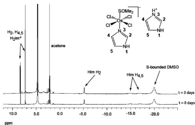
Figure 12. ^1\text{H} NMR spectra of 6 (5.5 mM) in phosphate buffer (0.05 M phosphate, 0.15 M NaCl, pH 7.4, 37^\circ\text{C} for t = 0 and 3 days with chemical formula and atom numbering scheme. For signal integration, acetone (1 \mu\text{L/mL} ) was added to the buffer solution as reference (2.16 ppm).
