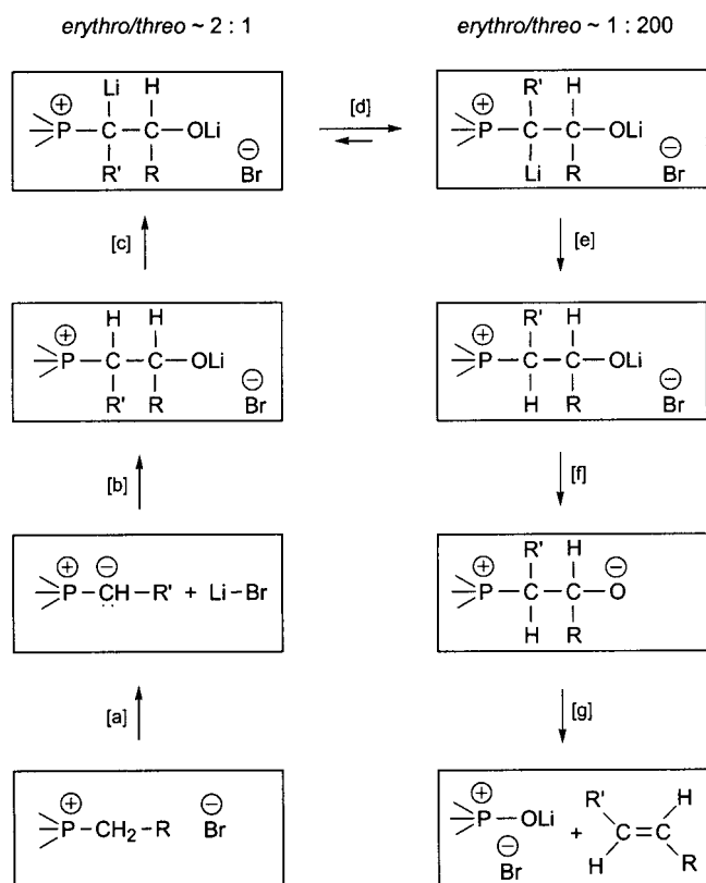
Scheme 2. The multistep, if one-pot protocol for trans -selective olefin formation. a) Lithium bromide containing phenyllithium (or any other organolithium) in THF and diethyl ether. b) Aldehyde \text{R}-\text{CH}=\text{O} . c) Lithium bromide containing phenyllithium in diethyl ether. d) Either 1 min at 25^\circ\text{C} or 30 min at -75^\circ\text{C} . e) Hydrogen chloride (1.0 equiv) in diethyl ether at -75^\circ\text{C} . f) Potassium tert -butoxide. g) Some 15 min at -25^\circ\text{C} .
