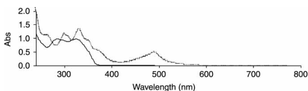
Figure 3. UV–vis spectra of \text{dU}^{\text{terpy}} 2 (solid line) and ( \text{dU}^{\text{terpy}} ) \text{Ru}(\text{terpy}) 3 (dashed line) ( c = 2.22 \times 10^{-5} \text{ M} in acetonitrile).
