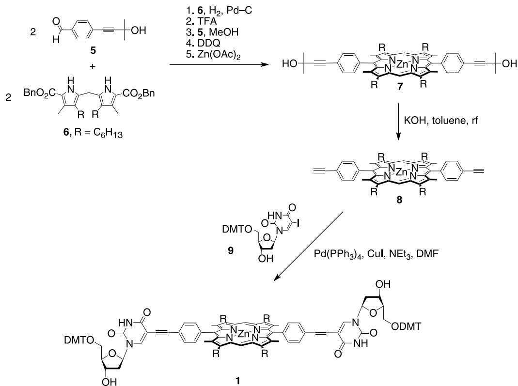
Scheme 1. Synthesis of 1 .
