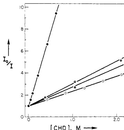
Figure 1. CHD quenching of DCA fluorescence in degassed pyridine (●), benzene (○), 0.99 M pyridine in benzene (●), 1.99 M pyridine in benzene (●); 25.0 ^\circ\text{C} .
