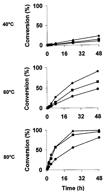
Figure 3. Effects of acyl donor and temperature on the time course of formation of sitostanyl oleate by esterification of 100 \mu mol of sitostanol with 300 \mu mol of oleic acid (●) and by transesterification of 100 \mu mol of sitostanol with 300 \mu mol of methyl oleate (◆) or 150 \mu mol of triolein (■) catalyzed by 50 mg of R. miehei lipase (Lipozyme IM) in vacuo at 40, 60, and 80 °C for various periods.
