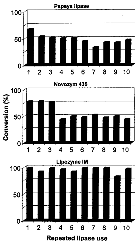
Figure 8. Percent conversion of sitostanol to sitostanyl oleate in the transesterification of sitostanol (100 \mu mol) with methyl oleate (300 \mu mol), catalyzed by papaya ( Cr. papaya ) latex lipase (50 mg), Cd. antarctica lipase B (Novozym 435, 50 mg), or R. miehei lipase (Lipozyme IM, 50 mg) after repeated use of the lipase catalyst as described under Experimental Procedures. The reactions were carried out in vacuo at 80 °C for 24 h.
