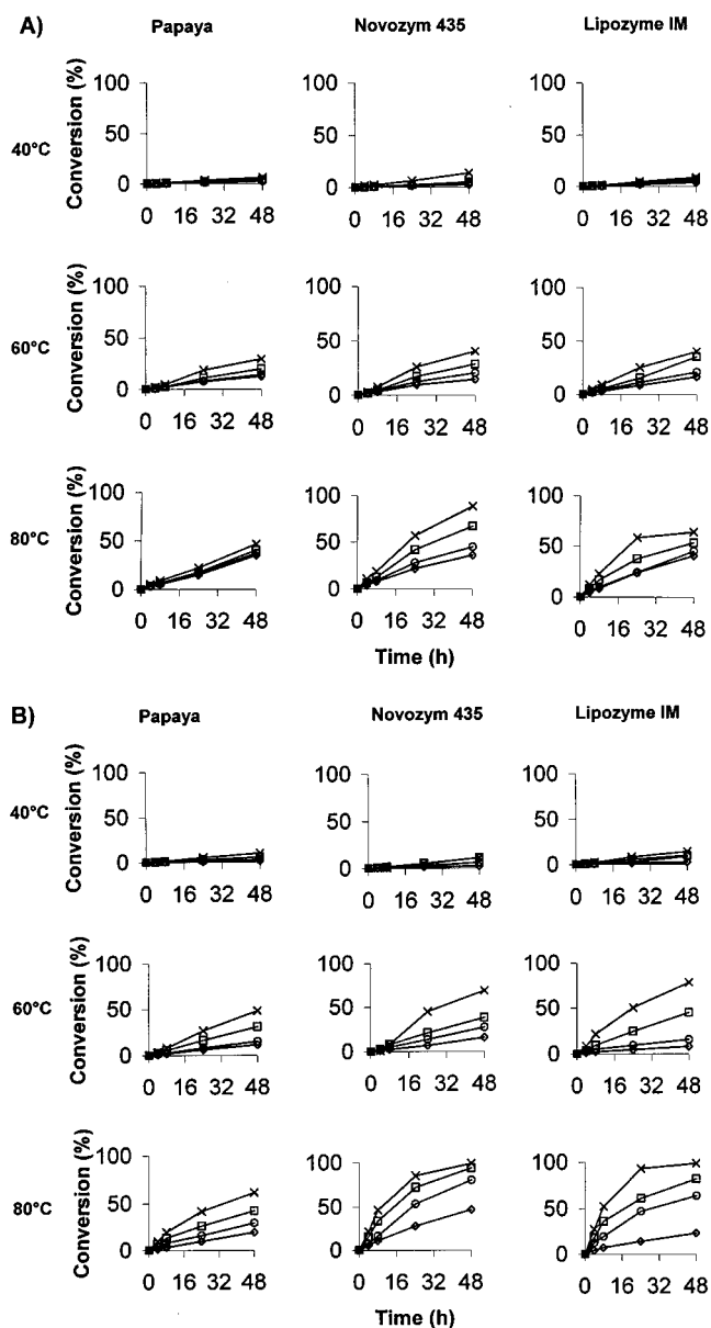
Figure 2. Time course of the formation of sitostanyl oleate via (A) esterification of 300 \mu mol of oleic acid or (B) transesterification of 300 \mu mol of methyl oleate with 100 \mu mol, each, of sitostanol catalyzed by various amounts ( \diamond , 6.25 mg; \square , 12.5 mg; \times , 50 mg) of different lipases [left, papaya ( Cr. papaya ) latex; center, Cd. antarctica lipase B (Novozym 435); right, R. miehei lipase (Lipozyme IM)] in vacuo at 40, 60, and 80 °C for various periods.
