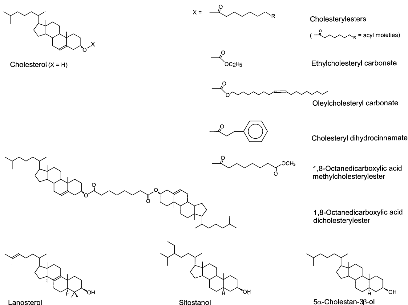
Figure 1. Chemical structures of steryl and stanlyl esters.
