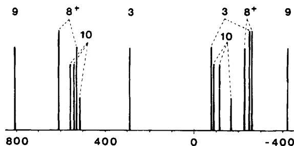
Figure 11. Comparison of the signals of the ring-C atoms (negative shifts) and of C \alpha (positive shifts) for [Cp*Cr(C 6 Me 6 )] + ( 8 + ), Cp*Cr(C 6 H 6 ) ( 3 ), Cp* 2 Cr ( 9 ), and [(EtMe 4 C 5 ) 2 Mn] + ( 10 ) at 305 K. The scale is in ppm. The relative intensities refer to six- and five-membered rings or to the symmetry-related signal splitting of 10 .
