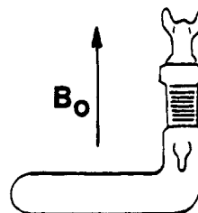
Figure 12. NMR tube used with solenoid probe heads. B_0 = direction of the magnetic induction.
