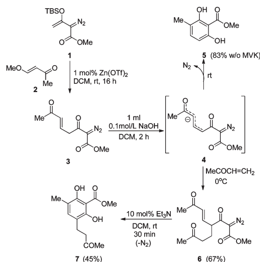
Scheme 1 Synthesis of 4-substituted-6-methyl-2-carboalkoxyresorcinols from methyl vinyl ketone. 11
