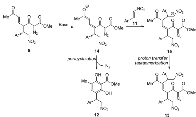
Scheme 2 Proposed pathway from 9 to resorcinols 12 and the bis-Michael addition products 13 .
