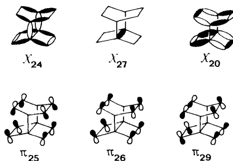
Fig. 3. Schematic representation of the most important precanonical MO's of 2 responsible for the \pi/\sigma interaction
