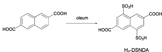
Scheme 1. Preparation of the H 4 -DSNDA Ligand
