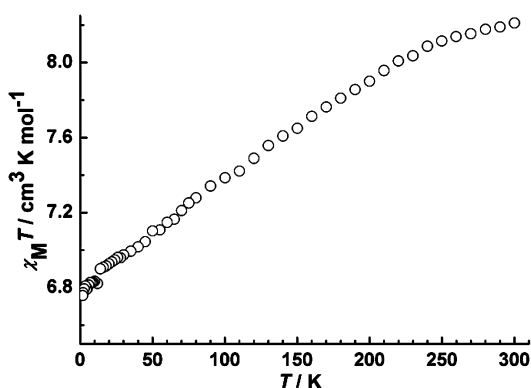
Figure 15. Temperature dependence of the \chi_M T product at 0.1 kOe for Gd(6).
