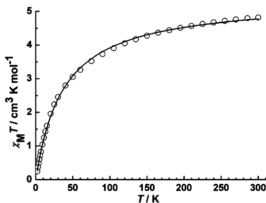
Figure 11. Temperature dependence of the \chi_M T product at 1 kOe for Pr(1). Solid line is the best fit obtained with the model as described in the text.
