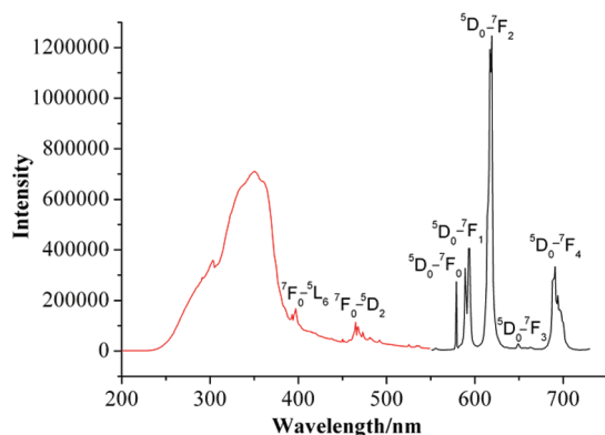
Figure 10. Room-temperature excitation (red) with emission monitored at approximately 618 nm, and emission (black) spectra for compound Eu(5) ( \lambda_{\text{ex}} = 350 nm) in the solid state.
