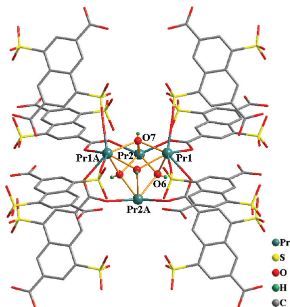
Figure 2. Tetranuclear [\text{Pr}_4(\mu_3\text{-OH})_4] SBU surrounded by eight \text{DSND4}^{4-} ligands.
