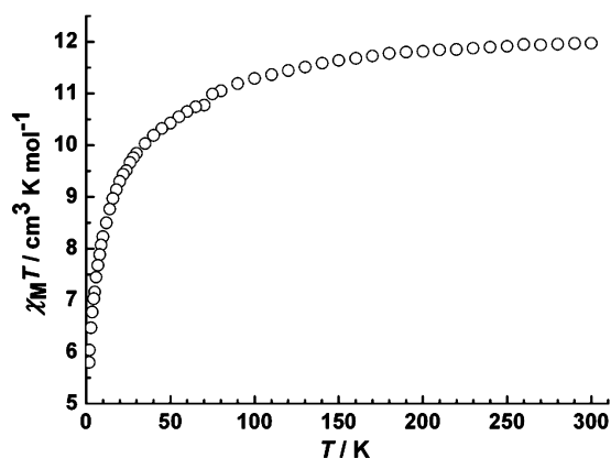
Figure 17. Temperature dependence of the \chi_M T product at 0.1 kOe for Er(8).
