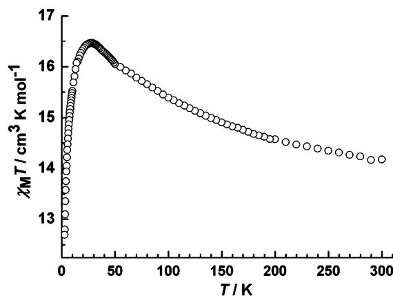
Figure 16. Temperature dependence of the \chi_M T product at 1 kOe for Dy(7).
