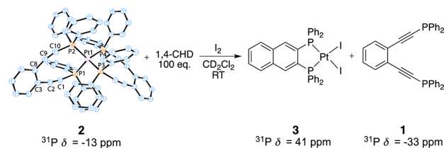
Scheme 2. Redox-Mediated Bergman Cyclization of 2 in the Presence of Excess 1,4-CHD To Yield the Benzannulated Product 3 a
