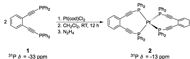
Scheme 1. Synthesis of Bis(1,2-bis((diphenylphosphino)ethynyl)benzene)platinum(0), 2
