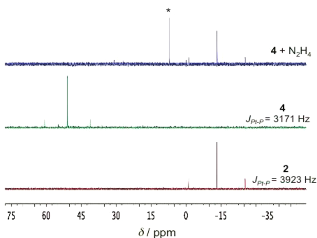
Figure 2. ^{31}\text{P} NMR spectra showing the oxidation of 2 to 4 and subsequent reduction of 4 to regenerate starting material. The designated (*) signal corresponds to the phosphine-oxide analogue of the free ligand, 6 , which is generated during the reduction reaction and has been confirmed and characterized by independent synthesis.
