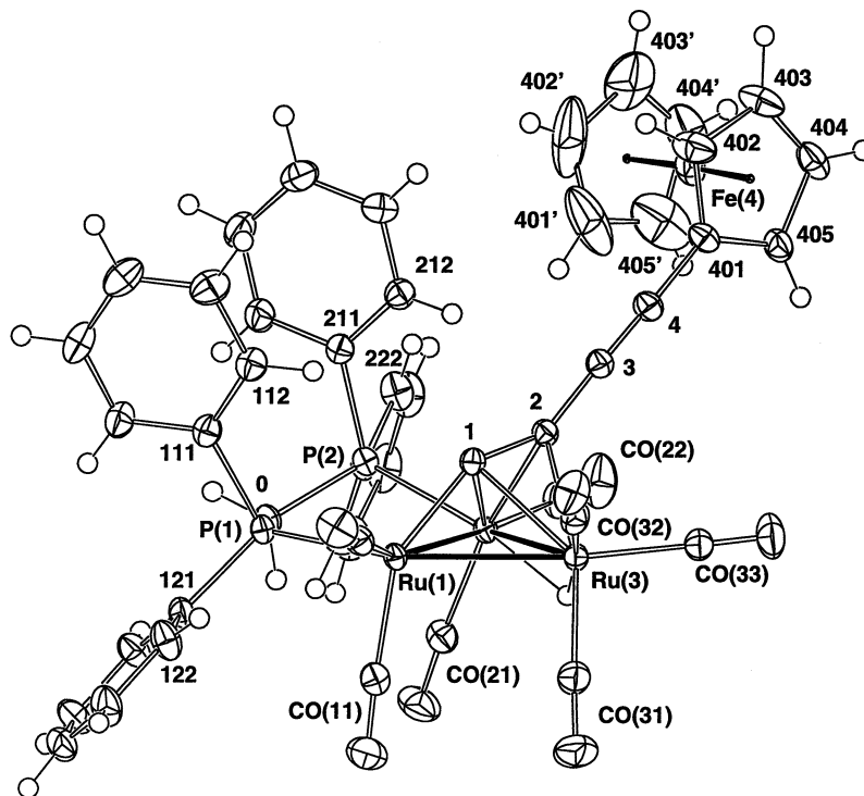
Fig. 3. Plot of a molecule of \text{Ru}_3(\mu\text{-H})(\mu_3\text{-C}_2\text{C}\equiv\text{CFc})(\mu\text{-dppm})(\text{CO})_7 ( 3 ).
