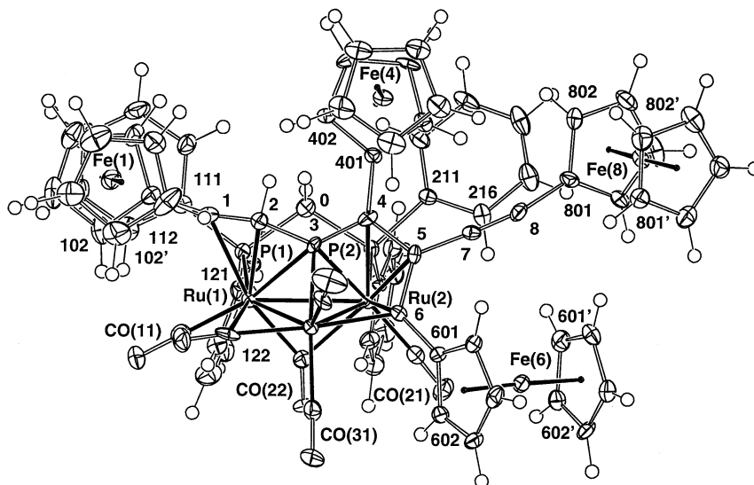
Fig. 4. Plot of a molecule of \text{Ru}_3\{\mu_3\text{-FcCC}(\text{C}\equiv\text{CFc})\text{CFcC}(\text{C}\equiv\text{CFc})\}(\mu\text{-dppm})(\mu\text{-CO})_2(\text{CO})_4 ( 7 ).
