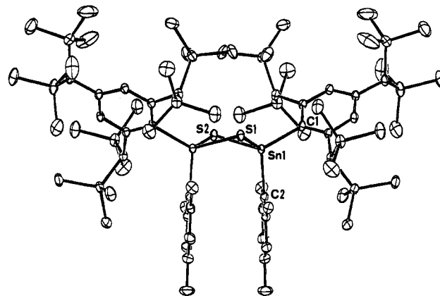
Figure 3. ORTEP drawing of cis -[Tb(Mes)SnS] 2 (27a) with thermal ellipsoid plot (20% probability).
