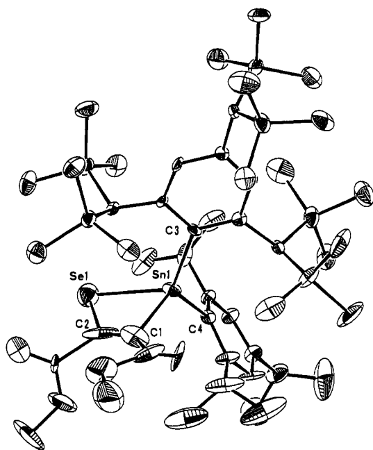
Figure 7. ORTEP drawing of 1,2-selenastannete (14) with thermal ellipsoid plot (30% probability).
