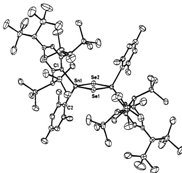
Figure 2. ORTEP drawing of trans -[Tb(Mes)SnSe] 2 (26b) with thermal ellipsoid plot (20% probability).
