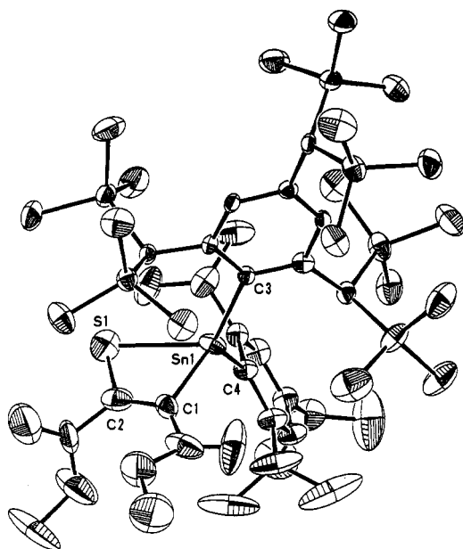
Figure 6. ORTEP drawing of 1,2-thiastannete (8) with thermal ellipsoid plot (30% probability).
