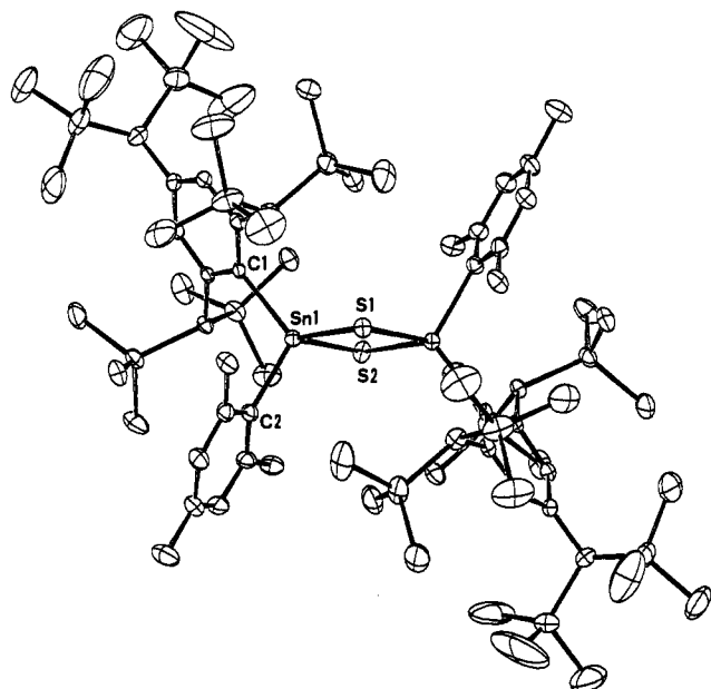
Figure 1. ORTEP drawing of trans -[Tb(Mes)SnS] 2 (26a) with thermal ellipsoid plot (20% probability).
