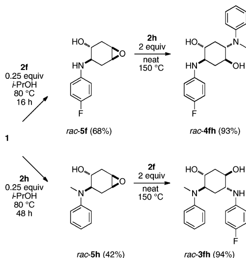
Scheme 3. Regiocontrolled Route to Unsymmetrical 1,3- or 1,4-Diols
