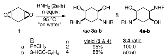
Scheme 1. Opening of trans -Diepoxide 1 with Benzylamine 2a and 3-Ethynylaniline 2b
