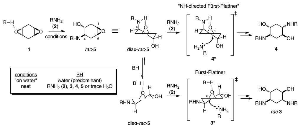
Scheme 2. Proposed Mechanistic Pathways for Formation of 1,3- and 1,4-Diols ( 3 and 4 , Respectively)
