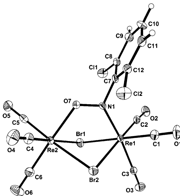
Figure 2. Molecular structure of 6b . Selected bond lengths [Å] and angles [°]: Re(1)–N(1) 1.990(6), Re(2)–O(7) 2.116(5), Re(1)–Br(1) 2.6115(13), Re(1)–Br(2) 2.5965(11), Re(2)–Br(1) 2.6199(10), Re(2)–Br(2) 2.6305(12), O(7)–N(1) 1.299(8), N(1)–C(7) 1.451(9), Re(1)–C(1) 1.923(9), Re(1)–C(2) 1.936(9), Re(1)–C(3) 2.020(9), Re(2)–C(4) 1.902(8), Re(2)–C(5) 1.891(9), Re(2)–C(6) 1.907(9); N(1)–O(7)–Re(2) 121.8(4), O(7)–N(1)–Re(1) 126.5(5), O(7)–Re(2)–Br(2) 84.25(14), O(7)–Re(2)–Br(1) 83.58(4), N(1)–Re(1)–Br(1) 85.84(17), N(1)–Re(1)–Br(2) 86.73(17), Br(2)–Re(1)–Br(1) 82.89(4), Br(1)–Re(2)–Br(2) 82.07(4), O(7)–N(1)–C(7) 109.7(5), O(7)–N(1)–C(12) 85.44.
