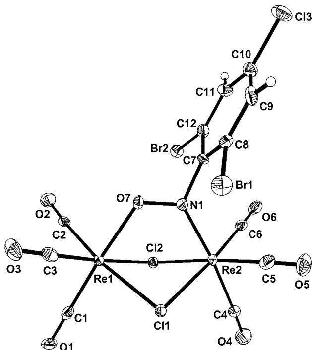
Figure 5. Molecular structure of 8a . Selected bond lengths [Å] and angles [°]: Re(2)–N(1) 2.007(8), Re(1)–O(7) 2.099(6), Re(1)–Cl(2) 2.497(3), Re(1)–Cl(1) 2.500(2), Re(2)–Cl(2) 2.474(2), Re(2)–Cl(1) 2.482(2), O(7)–N(1) 1.297(10), N(1)–C(7) 1.440(11), Re(1)–C(1) 1.920(11), Re(1)–C(2) 1.927(10), Re(1)–C(3) 1.899(11), Re(2)–C(4) 2.018(10), Re(2)–C(5) 1.934(12), Re(2)–C(6) 1.941(11); N(1)–O(7)–Re(1) 120.8(5), O(7)–N(1)–Re(2) 123.3(6), O(7)–Re(1)–Cl(1) 83.50(18), O(7)–Re(1)–Cl(2) 83.67(18), N(1)–Re(2)–Cl(2) 85.4(2), N(1)–Re(2)–Cl(1) 85.0(2), Cl(2)–Re(1)–Cl(1) 79.27(8), Cl(2)–Re(2)–Cl(1) 80.06(8), O(7)–N(1)–C(7) 110.9(7), O(7)–N(1)–C(7)–C(12) 84.84.
