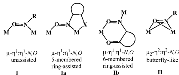
Scheme 1. Bonding modes of C -nitroso compounds bridging two metals ( \mu - \eta^2 - N,O ).
