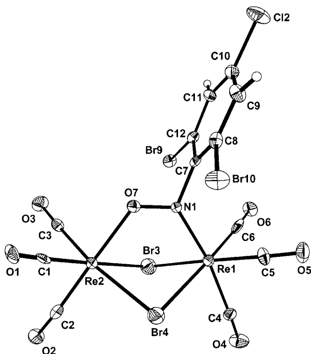
Figure 6. Molecular structure of 8b . Selected bond lengths [Å] and angles [°]: Re(1)–N(1) 2.001(12), Re(2)–O(7) 2.127(11), Re(1)–Br(3) 2.578(2), Re(1)–Br(4) 2.611(2), Re(2)–Br(3) 2.589(2), Re(2)–Br(4) 2.637(2), O(7)–N(1) 1.257(15), N(1)–C(7) 1.458(19), Re(2)–C(1) 1.963(19), Re(2)–C(2) 1.95(2), Re(2)–C(3) 1.903(17), Re(1)–C(4) 2.08(2), Re(1)–C(5) 1.908(19), Re(1)–C(6) 1.99(2); N(1)–O(7)–Re(2) 123.7(9), O(7)–N(1)–Re(1) 123.3(10), O(7)–Re(2)–Br(3) 83.5(3), O(7)–Re(2)–Br(4) 83.5(3), N(1)–Re(1)–Br(3) 86.6(3), N(1)–Re(1)–Br(4) 86.4(4), Br(3)–Re(1)–Br(4) 81.10(7), Br(3)–Re(2)–Br(4) 80.40(7), O(7)–N(1)–C(7) 109.9(11), O(7)–N(1)–C(7)–C(12) 83.49.
