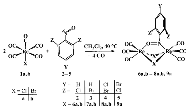
Scheme 2. Synthesis of sterically hindered \mu_2\text{-(}\eta^2\text{-N,O)} -nitrosobenzene complexes 6–9 .
