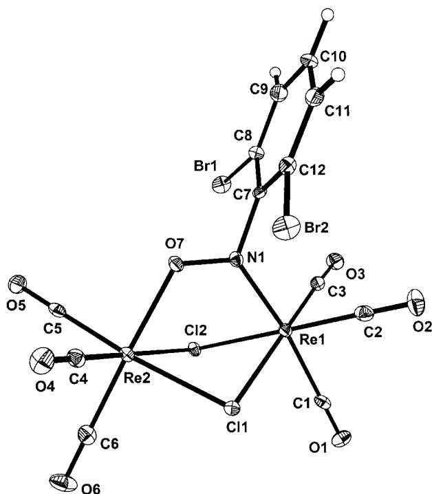
Figure 3. Molecular structure of 7a . Selected bond lengths [Å] and angles [°]: Re(1)–N(1) 1.991(4), Re(2)–O(7) 2.126(4), Re(1)–Cl(1) 2.4801(12), Re(1)–Cl(2) 2.5000(12), Re(2)–Cl(1) 2.5117(12), Re(2)–Cl(2) 2.5144(11), O(7)–N(1) 1.282(5), N(1)–C(7) 1.460(7), Re(1)–C(1) 2.030(6), Re(1)–C(2) 1.923(6), Re(1)–C(3) 1.930(6), Re(2)–C(4) 1.903(5), Re(2)–C(5) 1.914(6), Re(2)–C(6) 1.920(6); N(1)–O(7)–Re(2) 120.3(3), O(7)–N(1)–Re(1) 126.2(3), O(7)–Re(2)–Cl(2) 82.82(9), O(7)–Re(2)–Cl(1) 83.78(11), N(1)–Re(1)–Cl(1) 86.47(12), N(1)–Re(1)–Cl(2) 84.65(12), Cl(2)–Re(1)–Cl(1) 80.87(4), Cl(1)–Re(2)–Cl(2) 79.98(5), O(7)–N(1)–C(7) 109.9(4), O(7)–N(1)–C(7)–C(12) 85.28.
