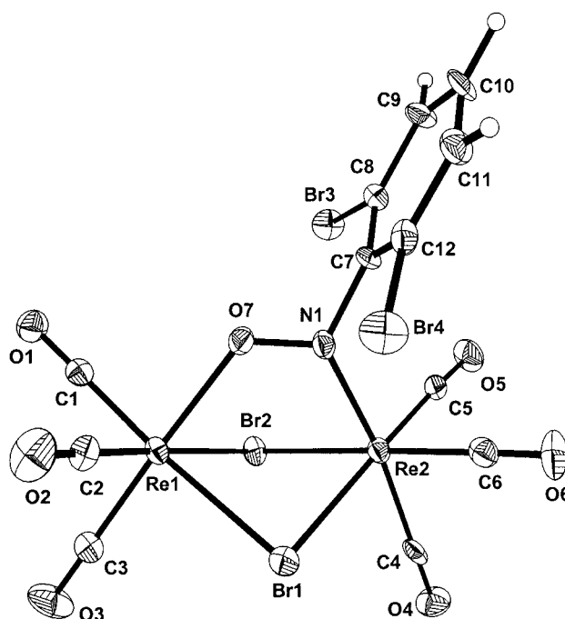
Figure 4. Molecular structure of 7b . Selected bond lengths [Å] and angles [°]: Re(2)–N(1) 2.012(8), Re(1)–O(7) 2.123(7), Re(1)–Br(1) 2.6364(10), Re(1)–Br(2) 2.6292(10), Re(2)–Br(1) 2.6057(10), Re(2)–Br(2) 2.6182(10), O(7)–N(1) 1.279(9), N(1)–C(7) 1.453(12), Re(1)–C(1) 1.874(11), Re(1)–C(2) 1.902(10), Re(1)–C(3) 1.936(12), Re(2)–C(4) 2.043(12), Re(2)–C(5) 1.920(11), Re(2)–C(6) 1.908(11); N(1)–O(7)–Re(1) 122.7(6), O(7)–N(1)–Re(2) 123.4(6), O(7)–Re(1)–Br(2) 83.53(16), O(7)–Re(1)–Br(1) 84.39(16), N(1)–Re(2)–Br(1) 87.1(2), N(1)–Re(2)–Br(2) 85.6(2), Br(1)–Re(1)–Br(2) 82.51(3), Br(2)–Re(2)–Br(1) 81.72(3), O(7)–N(1)–C(7) 110.9(7), O(7)–N(1)–C(7)–C(12) 84.91.
