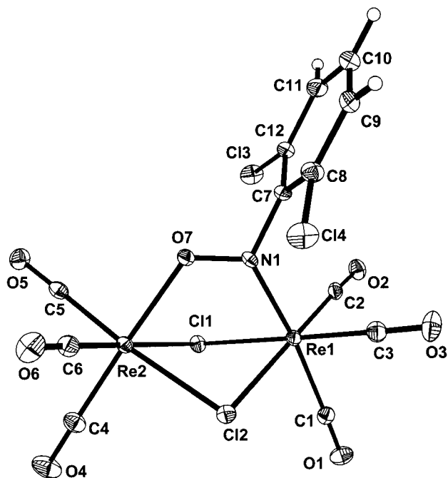
Figure 1. Molecular structure of 6a . Selected bond lengths [Å] and angles [°]: Re(1)–N(1) 1.994(4), Re(2)–O(7) 2.124(4), Re(1)–Cl(1) 2.4914(14), Re(1)–Cl(2) 2.4726(14), Re(2)–Cl(1) 2.5024(14), Re(2)–Cl(2) 2.5056(14), O(7)–N(1) 1.282(6), N(1)–C(7) 1.457(6), Re(1)–C(1) 2.031(6), Re(1)–C(2) 1.952(6), Re(1)–C(3) 1.917(7), Re(2)–C(4) 1.928(6), Re(2)–C(5) 1.902(6), Re(2)–C(6) 1.908(6); N(1)–O(7)–Re(2) 120.2(3), O(7)–N(1)–Re(1) 123.9(3), O(7)–Re(2)–Cl(2) 82.82, O(7)–Re(2)–Cl(1) 82.82(11), N(1)–Re(1)–Cl(1) 84.52(13), N(1)–Re(1)–Cl(2) 85.96(13), Cl(2)–Re(1)–Cl(1) 80.83(5), Cl(1)–Re(2)–Cl(2) 79.98(5), O(7)–N(1)–C(7) 110.3(4), O(7)–N(1)–C(8) 84.74.
