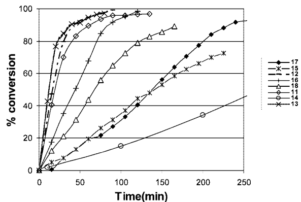
Figure 3. Reaction profile of conversion vs time for the hydrosilylation of n -BuC≡CH with different precursors.
