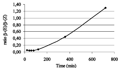
Figure 4. \beta\text{-(E)}/\beta\text{-(Z)} ratio for the hydrosilylation of n\text{-BuC}\equiv\text{CH} catalyzed by [\text{RhCl}(\text{cod})(t\text{-BuIm}(\text{CH}_2)_3\text{N}(\text{CH}_3)_2)] ( 13 ) at 60 °C. Total consumption of 1-hexyne at t = 120 min.
