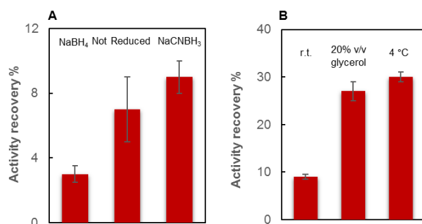
Figure 1. A) Effect of the reducing agent on the activity recovery (observed activity/starting activity)×100. B) Effect of glycerol and temperature on the activity recovery ( \text{NaCNBH}_3 ). These immobilization experiments were performed with 0.5 g of glyoxyl-agarose in a final volume of 5 mL by using the same protein loading ( 2 \text{ mg g}^{-1} ), activity loading ( 4.58 \text{ U g}^{-1} ) and run time (3 h). For the reduction step, 5 mg of the reducing agent were added and the mixture was stirred for further 30 min.
