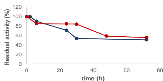
Figure 2. Stability of Vf -ATA immobilized on glyoxyl-agarose (blue) compared to free Vf -ATA (red). Experimental conditions: phosphate buffer (pH 8.0, 100 mM) containing DMSO (2% v/v) in the presence of 10 mM (S)-MBA and 1 mM PLP. Immobilized Vf -ATA: 50 mg, final volume: 1 mL; free Vf -ATA: 2.6 mg, final volume: 3 mL. The residual activity was determined by the spectrophotometric assay (see Experimental Section).
