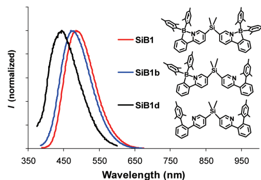
Figure 5. Normalized fluorescence spectra of SiB1 and its C–C coupled products.
