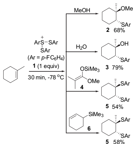
Scheme 2. The reactions of \text{ArS}(\text{ArSSAr})^+ ( 1 ) ( \text{Ar} = p\text{-FC}_6\text{H}_4 ) with 1-methylcyclohexene followed by addition of a quenching nucleophile.
