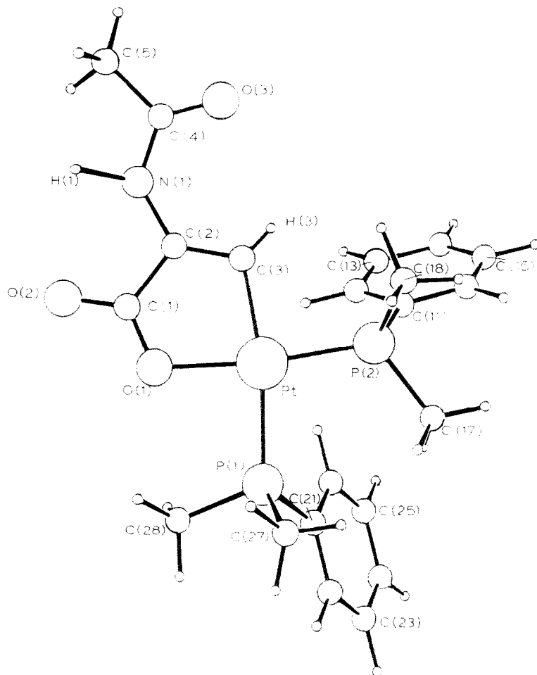
Fig. 1. Molecular structure of [Pt{CH=C(NHCOMe)C(O)O}(PMe 2 Ph) 2 ], 4c . Interatomic distances: Pt–P(1) 2.316(3), Pt–P(2) 2.207(2), Pt–O(1) 2.086(6), Pt–C(3) 2.027(11), C(2)–C(3) 1.331(13), C(1)–C(2) 1.498(14), C(1)–O(1) 1.267(11), C(1)–O(2) 1.244(10), C(2)–N(1) 1.420(12), N(1)–C(4) 1.346(15), C(4)–C(5) 1.498(15), C(4)–O(3) 1.233(13) Å. Angles: P(1)–Pt–P(2) 100.2(1), P(1)–Pt–O(1) 87.0(2), P(2)–Pt–C(3) 90.6(3), C(3)–Pt–O(1) 82.2(3), Pt–C(3)–C(2) 110.5(8), Pt–O(1)–C(1) 111.8(6), O(1)–C(1)–C(2) 117.0(8), C(1)–C(2)–C(3) 118.3(9)°.
