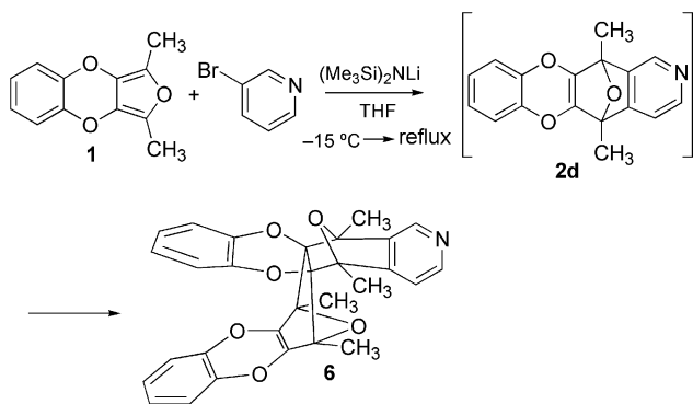
Scheme 3. Cycloaddition with 3,4-pyridyne.
