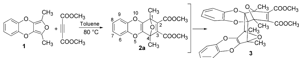
Scheme 1. Cycloaddition with DMAD.
