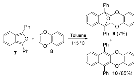
Scheme 4. Preparation of adducts from 1,4-benzodioxin.
