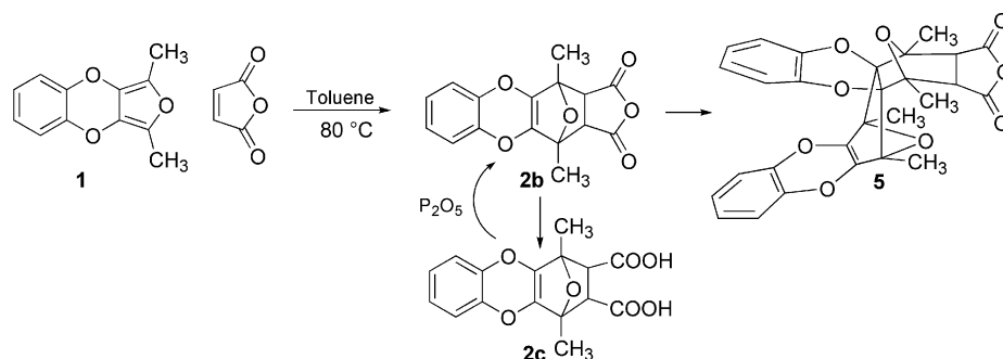
Scheme 2. Cycloaddition with maleic anhydride.
