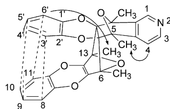
Figure 2. Correlation observed in the NOESY spectrum of bis-adduct 6 .
