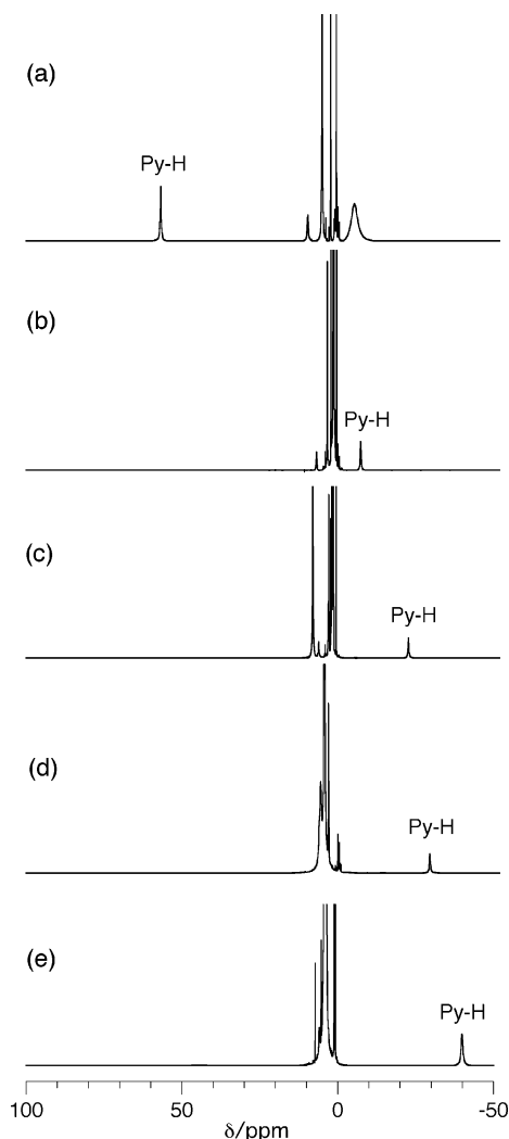
Figure 1. ^1\text{H} NMR spectra of \text{Fe}(\text{TiPrP})\text{L}_2^+ taken in \text{CD}_2\text{Cl}_2 solution at 298 K where L's are (a) 3,5- \text{Me}_2\text{PyNO} , (b) DMSO, (c) DMF, (d) MeOH, and (e) 1,4-dioxane. The broad signal at \delta -3.9 ppm in (a) is ascribed to the ligand protons.
