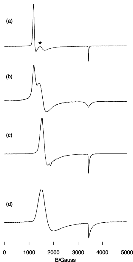
Figure 7. X-band EPR spectra of \text{Fe}(\text{OETPP})\text{L}_2^+ taken in frozen \text{CH}_2\text{Cl}_2 solution at 4.2 K, where L's are (a) 4-MePyNO, (b) PyNO, (c) DMF, and (d) MeOH. A small signal signified by * is ascribed to the minor component.
