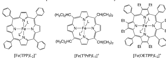
Scheme 1. Complexes Examined in This Study
