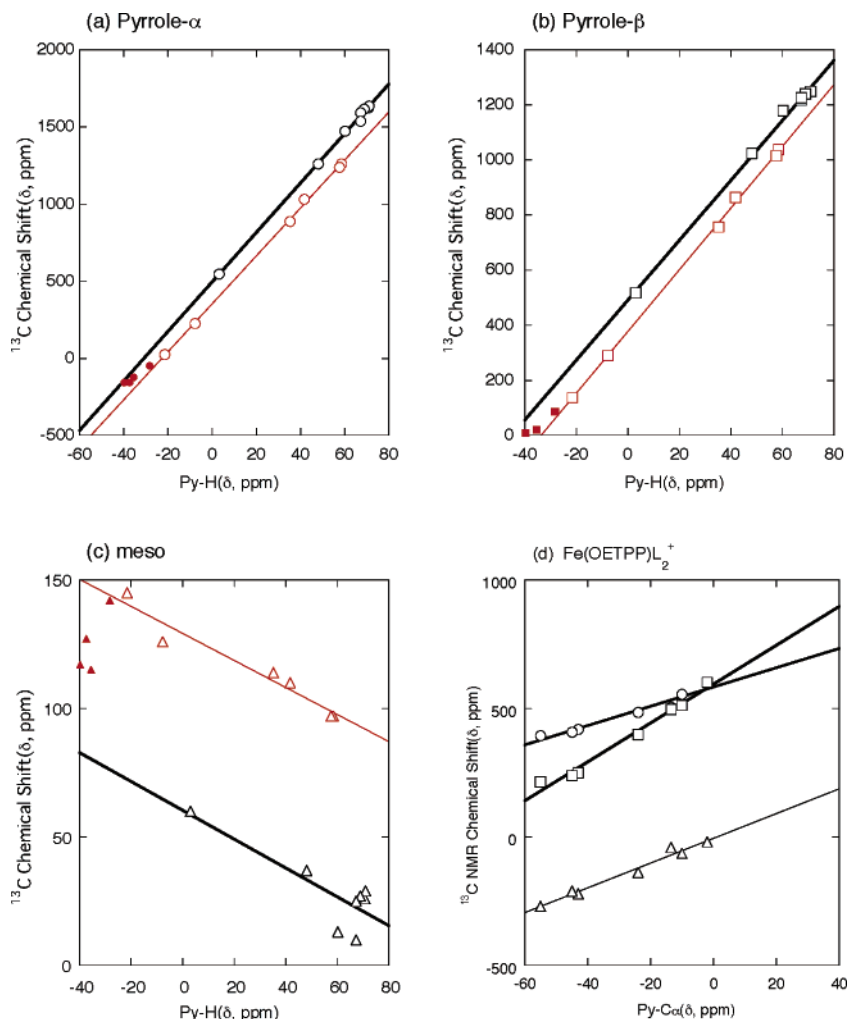
Figure 8. Chemical shift correlation. (a) Py-H vs Py- \alpha in Fe(TPP)L 2 + (black) and Fe(T'PrP)L 2 + (red), (b) Py-H vs Py- \beta in Fe(TPP)L 2 + (black) and Fe(T'PrP)L 2 + (red), (c) Py-H vs meso in Fe(TPP)L 2 + (black) and Fe(T'PrP)L 2 + (red), and (d) Py-C \alpha vs Py- \alpha (○), Py- \beta (□), and meso (Δ) in Fe(OETPP)L 2 + . The filled red marks in (a)–(c) correspond to the signals of Fe(T'PrP)L 2 + where L's are MeOH, THF, 2-MeTHF, and dioxane.
