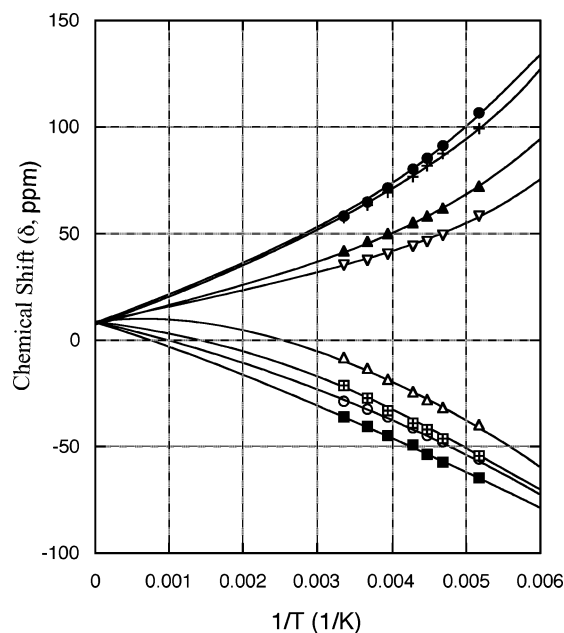
Figure 9. Curie plots of the pyrrole-H signals of \text{Fe}(\text{T}^i\text{PrP})\text{L}_2^+ : ●, 4-MePyNO; +, 3,5-Me 2 PyNO; ▲, PyNO; ▽, 4-ClPyNO; △, DMSO; □, DMF; ○, MeOH; ■, THF.
