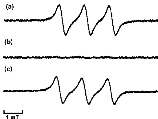
Figure 1. ESR spectra of solutions containing P-NAP (100 \mu M), FeSO_4 (1.5 mM), and N -methylglucamine dithiocarbamate (6 mM) (in PBS, pH 7.0, containing 1% DMF) after photoirradiation with UV-A (without attenuation) for 15 min. (a) A solution photoirradiated under an argon atmosphere. (b) A solution photoirradiated under aerobic conditions. (c) A solution containing SOD (1 kunit/mL) photoirradiated under aerobic conditions.
