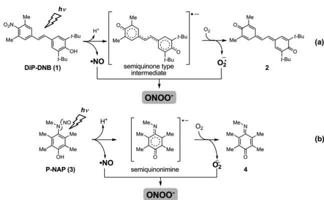
Chart 1. Photocontrollable ONOO − Generator and Proposed Mechanisms of ONOO − Release from DiP-DNB (a) and P-NAP (b)
