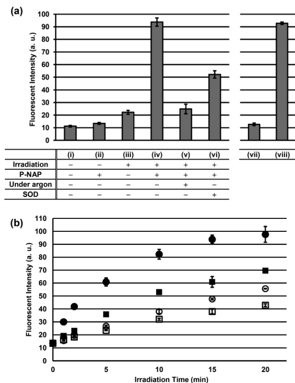
Figure 3. Fluorescence measurement for detection of \text{ONOO}^- generation using HKGreen-3. Samples contained P-NAP (10 \mu\text{M} ) and HKGreen-3 (10 \mu\text{M} ) in PBS, pH 7.4, with 0.2% DMF. The fluorescence intensity of sample solutions was determined at 535 nm with excitation at 520 nm. (a) The fluorescence intensity after irradiation of P-NAP with UV-A light (without attenuation) or incubation for 15 min: (i) solutions without P-NAP incubated in the dark; (ii) solutions including P-NAP incubated in the dark; (iii) solutions without P-NAP after irradiation; (iv) solutions including P-NAP after irradiation; (v) solutions including P-NAP after irradiation under an argon atmosphere; (vi) solutions including P-NAP and SOD (1 kunit/mL) after irradiation; (vii) solutions without SIN-1 incubated at 37 ^{\circ}\text{C} for 2 h; and (viii) solutions including SIN-1 (10 \mu\text{M} ) incubated at 37 ^{\circ}\text{C} for 2 h. p < 0.01 for (iv) versus (i)-(iii), (v), and (vi) by multiple t test ( n = 3 ). (b) Fluorescence intensity after irradiation of P-NAP for various time periods with various light intensities. Light intensity was not attenuated (●) or attenuated to 25% (■), 6% (○), or 1.5% (□). Error bars were calculated from three independent measurements.
