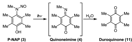
Chart 2. Expected Formation Pathway of Duroquinone, the Main Photodecomposition Product of P-NAP
