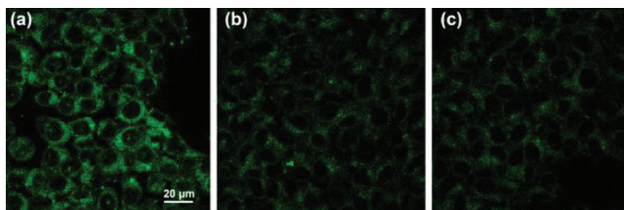
Figure 5. Fluorescence images of \text{ONOO}^- generation from P-NAP in HCT-116 cells in the presence of HKGreen-3A. Cultured HCT-116 cells were treated with HKGreen-3A (10 \mu\text{M} ) and P-NAP (10 \mu\text{M} ). The dishes were then photoirradiated with UV-A light (attenuated to 25%) or incubated in the dark for 15 min. The dishes were observed with a confocal microscope (a) after photoirradiation with P-NAP, (b) after incubation with P-NAP in the dark, and (c) after photoirradiation without P-NAP.
