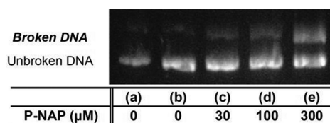
Figure 4. UV transillumination photograph of DNA strand-breaking assay after horizontal gel electrophoresis. Samples containing P-NAP and pBR322 plasmid DNA (0.04 mg/mL) in PBS (pH 7.0, containing 0.3% DMF) were photoirradiated with UV-A light (without attenuation) or incubated at room temperature in the dark for 15 min. (a) The solution after incubation in the dark without P-NAP. (b) The solution after irradiation without P-NAP. (c) The solution after irradiation with P-NAP (30 \mu\text{M} ). (d) The solution after irradiation with P-NAP (100 \mu\text{M} ). (e) The solution after irradiation with P-NAP (300 \mu\text{M} ).
