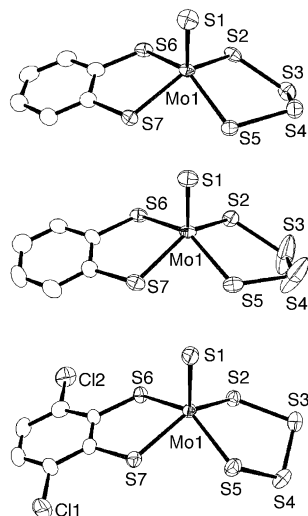
Figure 1. Crystal structures of the anionic complexes of (\text{Et}_4\text{N})_2[\text{MoS}(\text{S}_4)(\text{bdt})] ( 2 , above), (\text{Ph}_4\text{P})_2[\text{MoS}(\text{S}_4)(\text{bdt})] \cdot \text{DMF} ( 2a·DMF , middle), and (\text{Ph}_4\text{P})_2[\text{MoS}(\text{S}_4)(\text{bdtCl}_2)] \cdot \text{DMF} ( 3a·DMF , below) shown with 50% ellipsoids. The hydrogen atoms were omitted for clarity.
