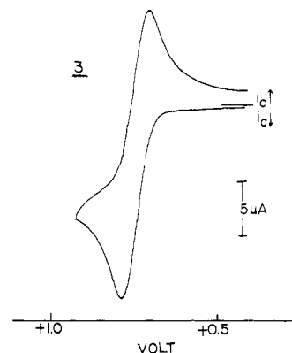
Figure 1. CV scan of (biphenyl) \text{Cr}(\text{CO})_3 ( 3 ) ( 4 \times 10^{-4}\text{ M} in \text{CH}_2\text{Cl}_2 at a Pt electrode, T = 263\text{ K} , v = 0.20\text{ V s}^{-1} ).
