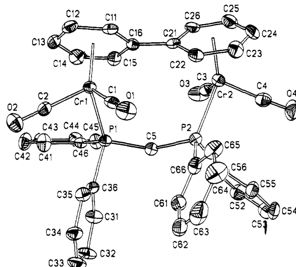
Figure 9. Molecular structure and atom labeling scheme for 8 .
