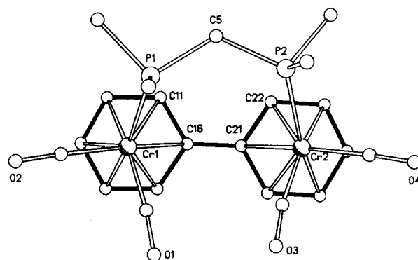
Figure 13. View of the staggering of the \text{Cr}(\text{CO})_2\text{P} units relative to the arene rings along the nearly parallel Cr-(ring centroid) vectors in 8 + .
