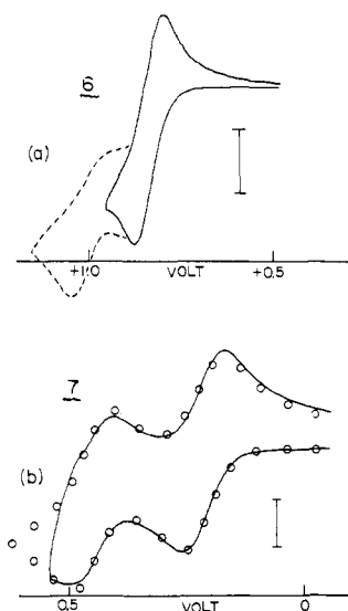
Figure 2. (a) CV scans of (biphenyl)[Cr(CO) 3 ] 2 ( 6 ) ( 4 \times 10^{-4} M in CH 2 Cl 2 at Pt, T = 260 K, v = 0.40 V s -1 ): solid line, scan through first wave only; dotted line, second wave included. (b) CV scan (solid line) of (biphenyl)[Cr(CO) 2 (PPh 3 ) 2 ] ( 7 ) 3 \times 10^{-4} M in CH 2 Cl 2 at Pt ( T = 273 K, v = 0.20 V s -1 ). Circles give calculated curves for reversible EE mechanism using E_1^\circ = +0.26 V and E_2^\circ = 0.52 V.
