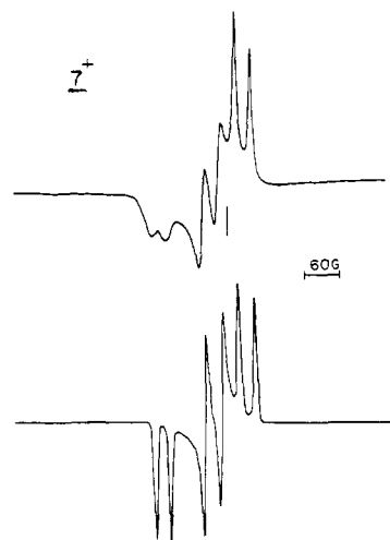
Figure 3. Experimental (top) and calculated (bottom) ESR spectra of 7 + (ca. 10^{-3} M) in a CH 2 Cl 2 /C 2 H 4 Cl 2 glass at 77 K. Parameters for the simulation are given in Table VI. The small vertical line gives the position of the dpph resonance.
