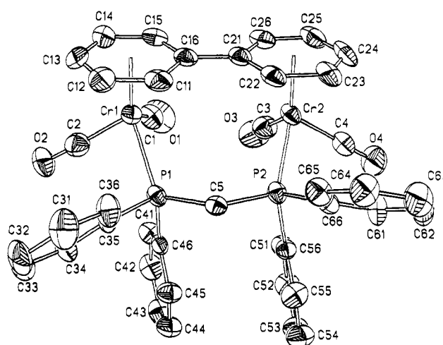
Figure 10. Molecular structure and atom labeling scheme for 8^+ .
