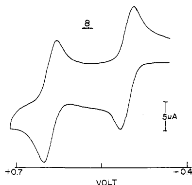
Figure 5. CV scan of (biphenyl) [\text{Cr}(\text{CO})_2]_2(\mu\text{-dppm}) ( 8 ) ( 3 \times 10^{-4} M in \text{CH}_2\text{Cl}_2 at Pt, T = 298 K, v = 0.20 V \text{s}^{-1} ).
