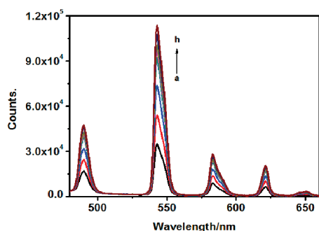
Figure 5. Emission spectra of the [\text{Tb} \cdot 1 \cdot 2]^{3+} complex ( 1 \times 10^{-5} \text{ M} ) upon addition of \text{K}^+ ( 0\text{--}1.3 \times 10^{-5} \text{ M} , from a to h) in \text{CH}_3\text{CN}/\text{CHCl}_3 (1:1, v/v) solution ( \lambda_{\text{ex}} = 340 \text{ nm} ).
