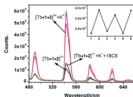
Figure 6. Emission spectral changes observed for [\text{Tb} \cdot 1 \cdot 2]^{3+} , [\text{Tb} \cdot 1 \cdot 2]^{3+} in the presence of \text{K}^+ , and [\text{Tb} \cdot 1 \cdot 2]^{3+} in the presence of \text{K}^+ and 18C6, respectively. Inset: the emission changes of [\text{Tb} \cdot 1]^{3+} ( 1 \times 10^{-5} \text{ M} ) in the presence of 2 ( 1 , 1.1 \times 10^{-5} \text{ M} ) and added \text{KPF}_6 ( 2 , 1.2 \times 10^{-5} \text{ M} ; 4 , 2.6 \times 10^{-5} \text{ M} ; 6 , 4.0 \times 10^{-5} \text{ M} ) and 18C6 ( 3 , 1.2 \times 10^{-5} \text{ M} ; 5 , 2.6 \times 10^{-5} \text{ M} ) in \text{CH}_3\text{CN}/\text{CHCl}_3 (1:1, v/v) solution at 544 \text{ nm} ( \lambda_{\text{ex}} = 340 \text{ nm} ).
