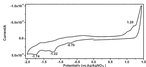
Figure 4. Cyclic voltammogram of [2]pseudorotaxane [\text{Tb} \cdot 1 \cdot 2]^{3+} in \text{CH}_2\text{Cl}_2 containing 0.1 M (t\text{-C}_4\text{H}_9)_4\text{NClO}_4 as the supporting electrolyte at 100 \text{ mVs}^{-1} ( [\text{Tb} \cdot 1 \cdot 2]^{3+} = 5 \times 10^{-4} \text{ M} , vs \text{Ag}/\text{AgNO}_3 ).
