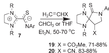
Scheme 5. The cycloaddition reactions between 7 and methyl acrylate or acrylonitrile.
