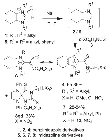
Scheme 2. Preparation of 2-aryl thiocarbamoyl benzimidazolium and imidazolinium inner salts.
