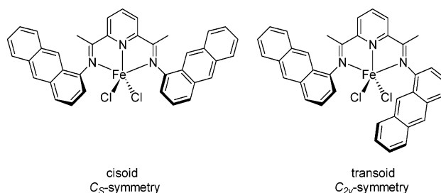
Figure 4. Possible conformations of complex 13.
