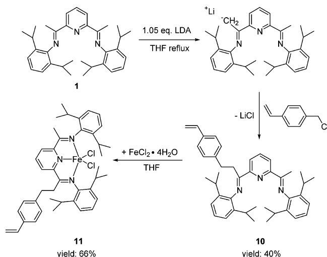
Scheme 2. Preparation of the Styrene-Substituted Complex 11
