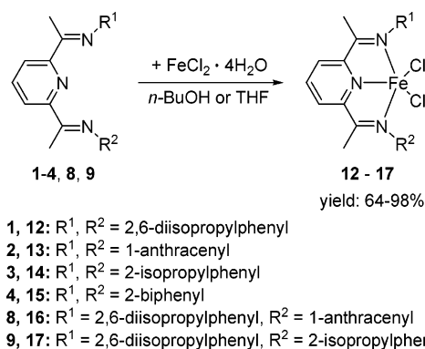
Scheme 3. Preparation of Bis(imino)pyridine-Substituted Iron(II) Complexes 12–17
