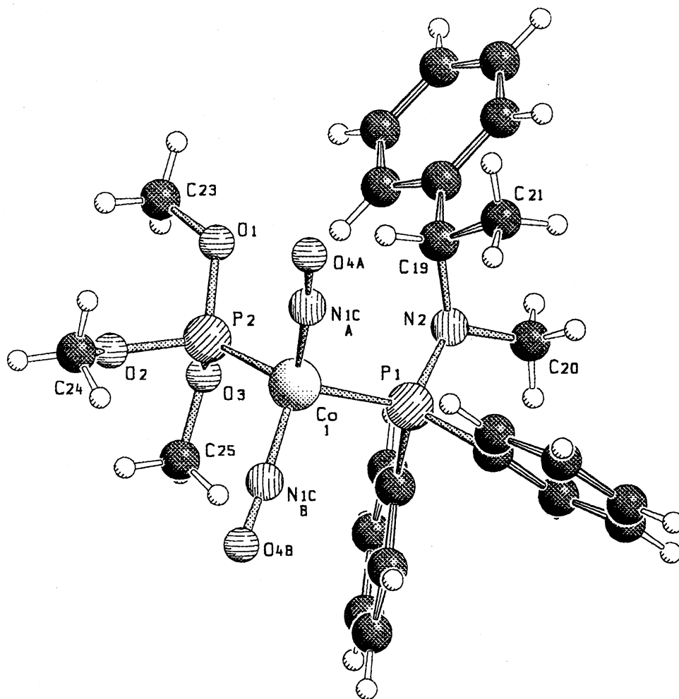
Fig. 1. SCHAKAL view of the molecular structure of \text{Co(CO)(NO)[P(OMe)}_3\text{]}[(S)\text{-PPh}_2\text{N(Me)CH(Me)(Ph)}] 1 . Only selected labels are shown for clarity [19].
