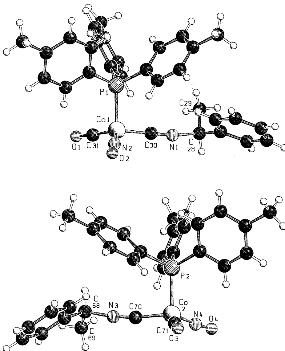
Fig. 3. SCHAKAL view of the molecular structures of the two independent molecules in the unit cell of (R_{Co}, S_C)\text{-Co(CO)(NO)[P}(p\text{-tolyl)}_3\text{][CNCH(Me)(Ph)] } \mathbf{3b} (above: P chirality of the propeller, bottom: M chirality). Only selected labels are shown for clarity.
