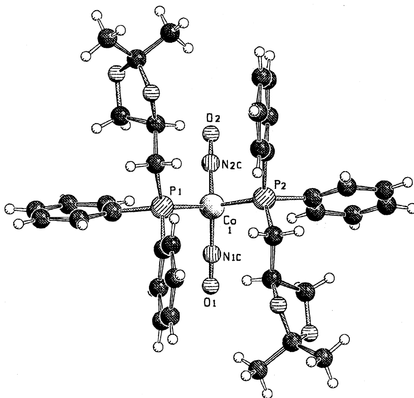
Fig. 4. SCHAKAL view of the molecular structure of \text{Co(CO)(NO)[(R)\text{-glyphos}]_2} 4 . Only selected labels are shown for clarity.
