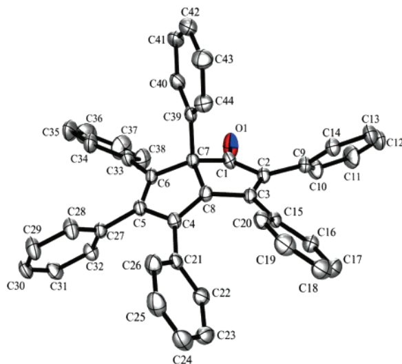
FIGURE 1. ORTEP representation of 5 .
