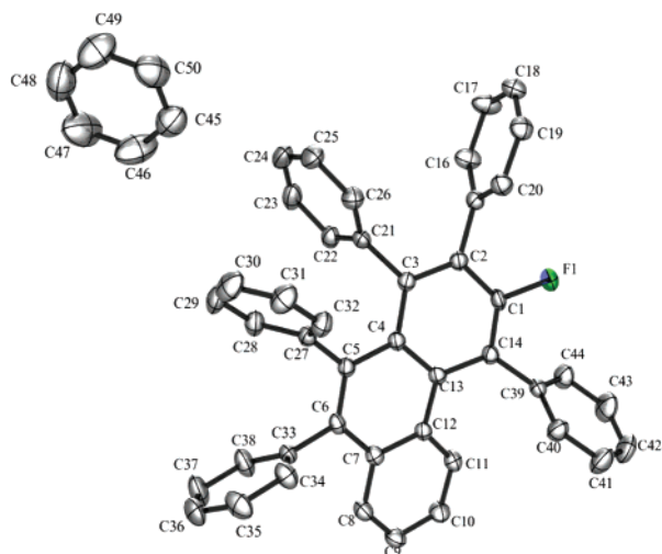
FIGURE 4. ORTEP representation of 9.
