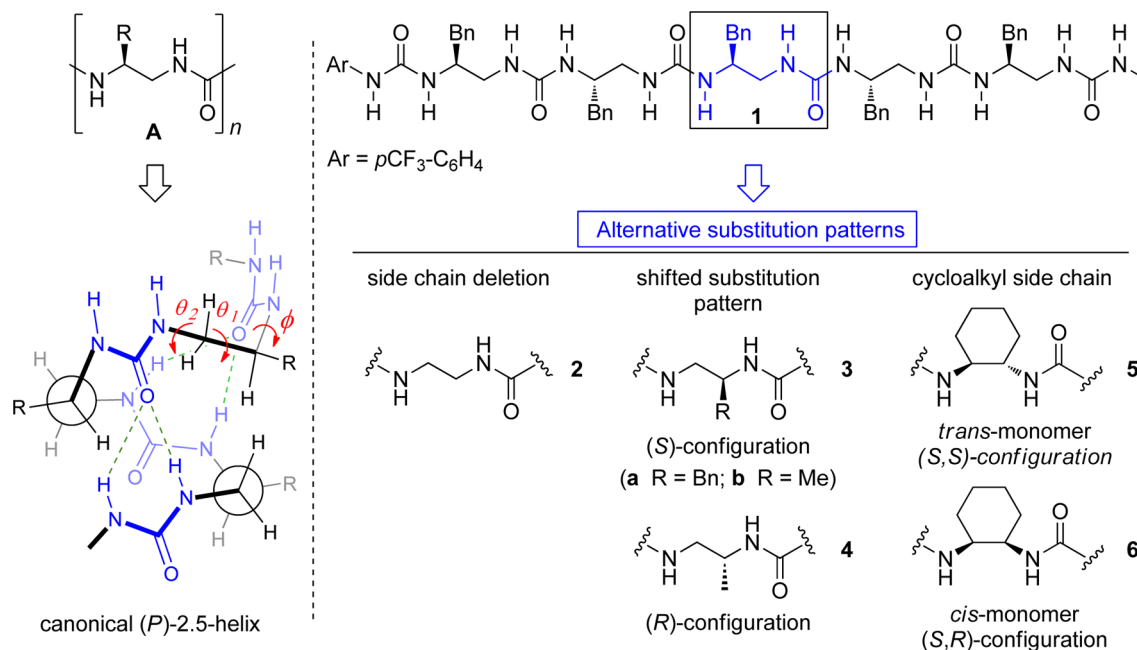
Figure 1. (left) Illustration of the canonical (P)-2.5-helical structure formed by N,N'-linked aliphatic oligoureas of type A together with the nomenclature used for the main-chain torsion angles: OC-N-C \beta -C \alpha is \phi , N-C \beta -C \alpha -N is \theta_1 , and C \beta -C \alpha -N-CO is \theta_2 . (right) Sequences of model urea pentamer 1 (canonical units with the S configuration) and the alternative substitution patterns evaluated in this study.
