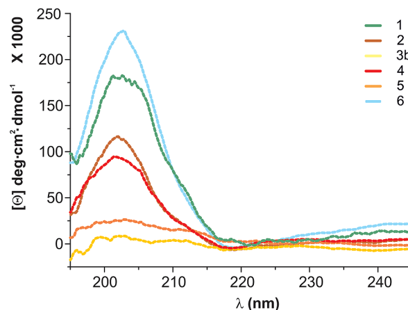
Figure 5. ECD spectra of oligoureas 1 – 6 ( 10^{-4} M in TFE) at 298 K.
