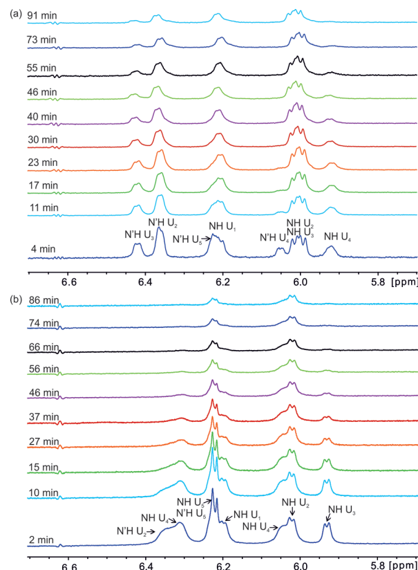
Figure 4. H/D exchange of backbone urea protons in (a) oligourea 1 and (b) oligourea 4 . The ^1\text{H} spectra (800 MHz) of the oligoureas ( 1 \text{ mM} in \text{CD}_3\text{OD} ) were recorded at 288 K.
