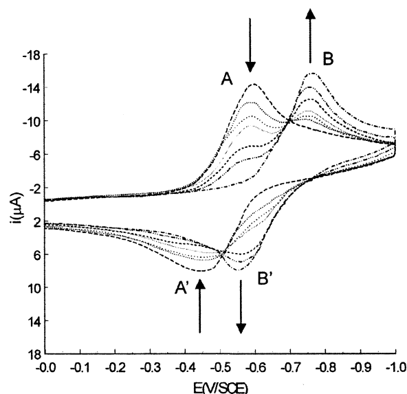
Figure 4. Cyclic voltammogram evolution of \text{Pd}_3(\text{CF}_3\text{CO}_2)^+ (0.5 mM) with 1 equiv of t -BuCOCl in THF with 0.2 M \text{NBu}_4\text{PF}_6 . Initial potential: 0 V. Scan rate: 100 \text{ mV s}^{-1} .
