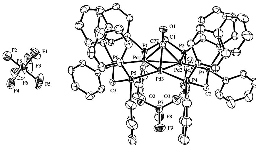
Figure 7. ORTEP drawing of [\text{Pd}_3(\text{dppm})_3(\text{CO})(\text{PF}_2\text{O}_2)](\text{PF}_6) . Toluene. The thermal ellipsoids are shown with 30% probability. The toluene solvation molecule and the H atoms are not shown for clarity.
