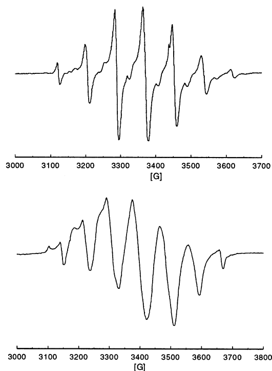
Figure 2. Experimental EPR spectrum of \text{Pd}_3^+ in THF at 293 K (top); experimental EPR spectrum of \text{Pd}_3^+ in THF at 100 K (bottom).
