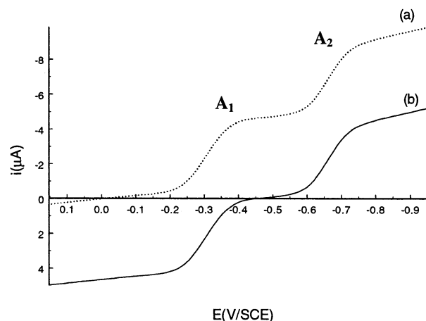
Figure 1. RDE voltammogram of 0.84 mM \text{Pd}_3(\text{PF}_6)_2 in THF. (a, dotted line) Alone; (b, solid line) after reduction with 0.2 M \text{NaBPh}_4 . Initial potential: +0.2 V. Scan rate: 20\text{ mV s}^{-1} .
