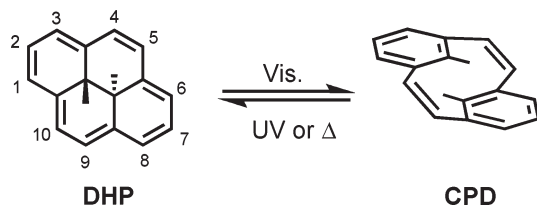
Chart 2. Optically Triggered Interconversion of the Dimethyldihydronaphthalene (DHP)/Cyclophanediene (CPD) System
