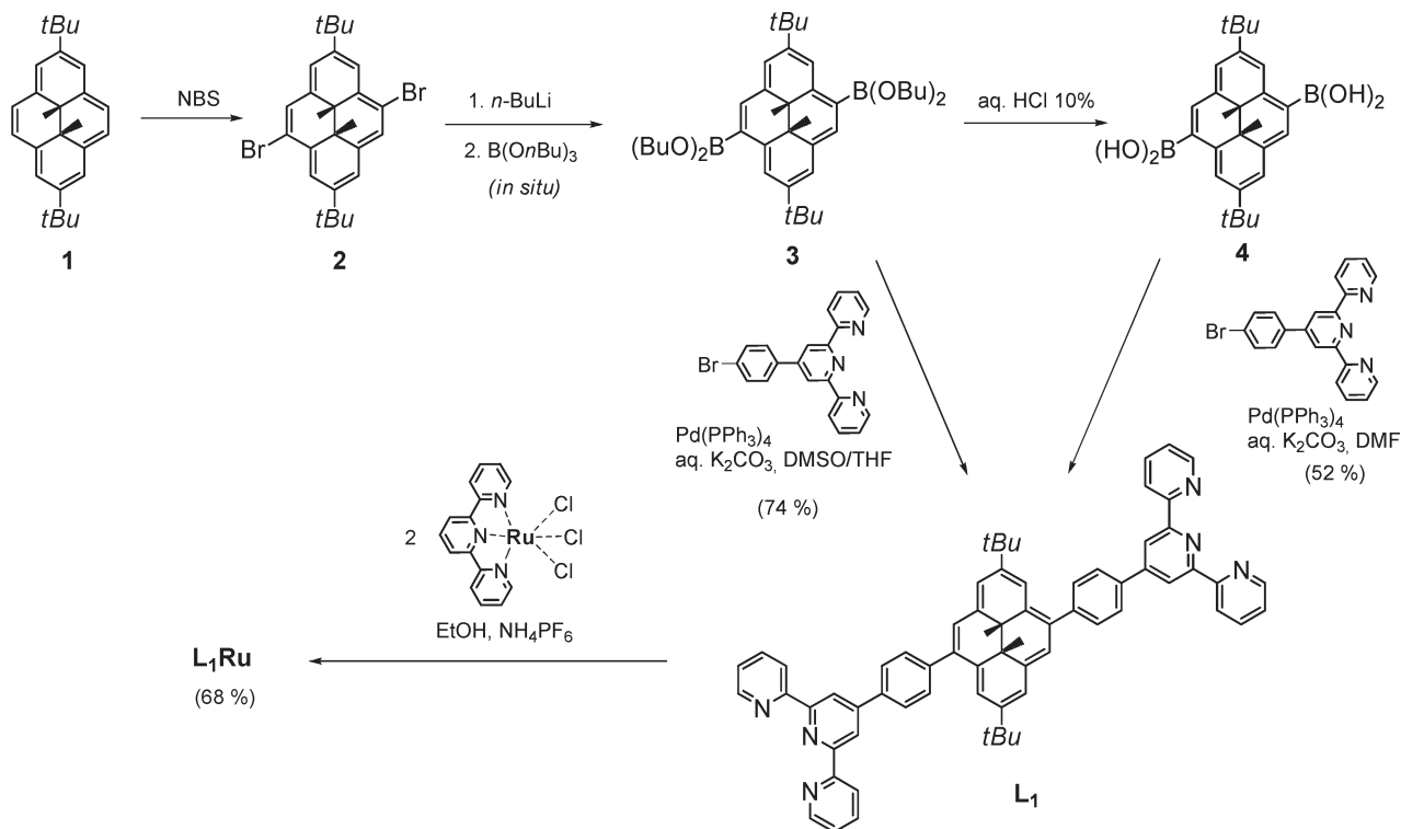
Scheme 1. Overall Synthetic Pathways for Preparation of L_1 via Suzuki Cross-Coupling Reaction and Preparation of L_1Ru
