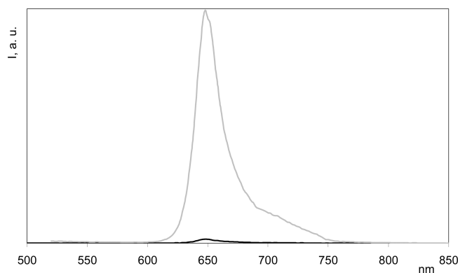
Figure 5. Emission spectra of L 2 Ru at room temperature in acetonitrile solution before (closed form; gray line) and after (open form; black line) irradiation at \lambda \geq 490 nm.
