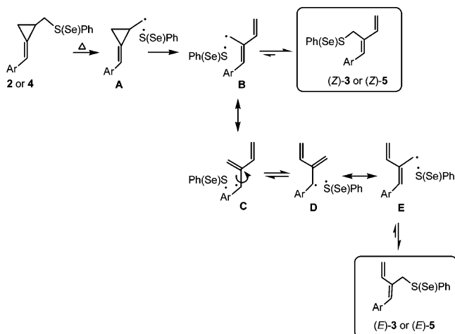
SCHEME 6. A Radical Rearrangement Mechanism Proposed for the Ring-Opening Transformation
