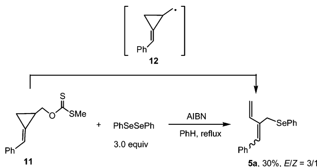
SCHEME 4. Control Experiment for This Radical Transformation
