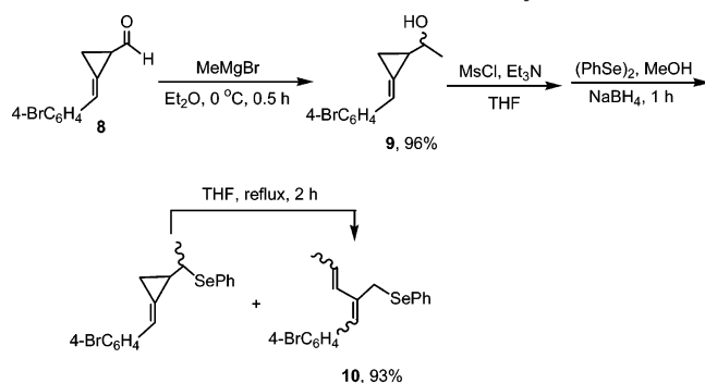
SCHEME 3. Formation of 5a via a Radical Process
