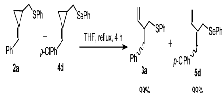
SCHEME 6. A Radical Rearrangement Mechanism Proposed for the Ring-Opening Transformation
