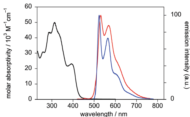
Chart 3. Absorption Spectrum [at 298 K in \text{CH}_2\text{Cl}_2 (black line)] and Emission Spectra [at 298 K in \text{CH}_2\text{Cl}_2 (red line) and 77 K in EPA glass (blue line)] of Complex 3 Containing Dicatena Ligands
