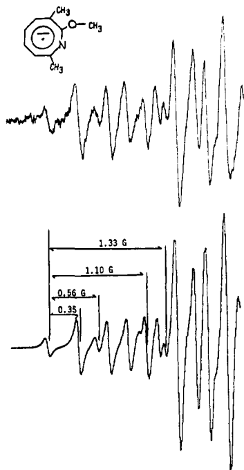
Figure 3. First few lines of the ESR spectrum of \text{DMMA}^{\bullet-} in HMPA at 25 °C. The lower spectrum is a computer simulation generated from the coupling constants indicated and a line width of 0.055 G.
