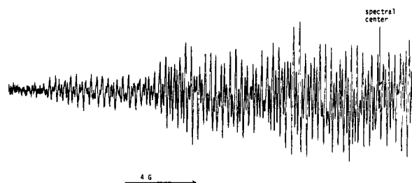
Figure 2. ESR spectrum of DMMA - at 0 °C. Only half of the spectrum is shown. The solvent is HMPA, and the arrow marks the center of the spectrum. Decomposition of the anion radical results in the high-field line intensities being smaller than predicted.
