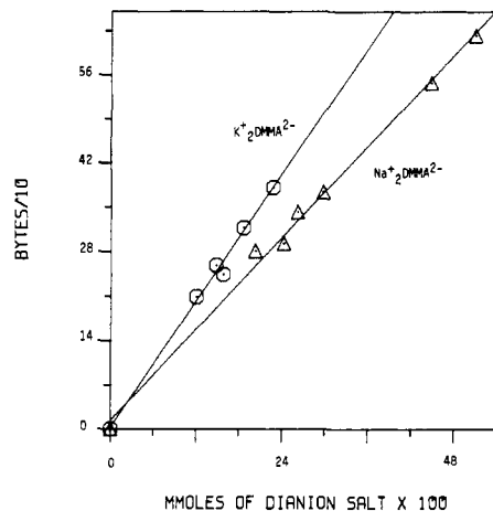
Figure 4. Plots of the change in the temperature of the calorimeter in computer bytes vs. the number of millimoles of DMMA dianion salts in the glass bulbs.
