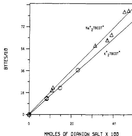
Figure 5. Plots of the change in the temperature of the calorimeter in computer bytes vs. the number of millimoles of TBCOT dianion salts in the glass bulbs.
