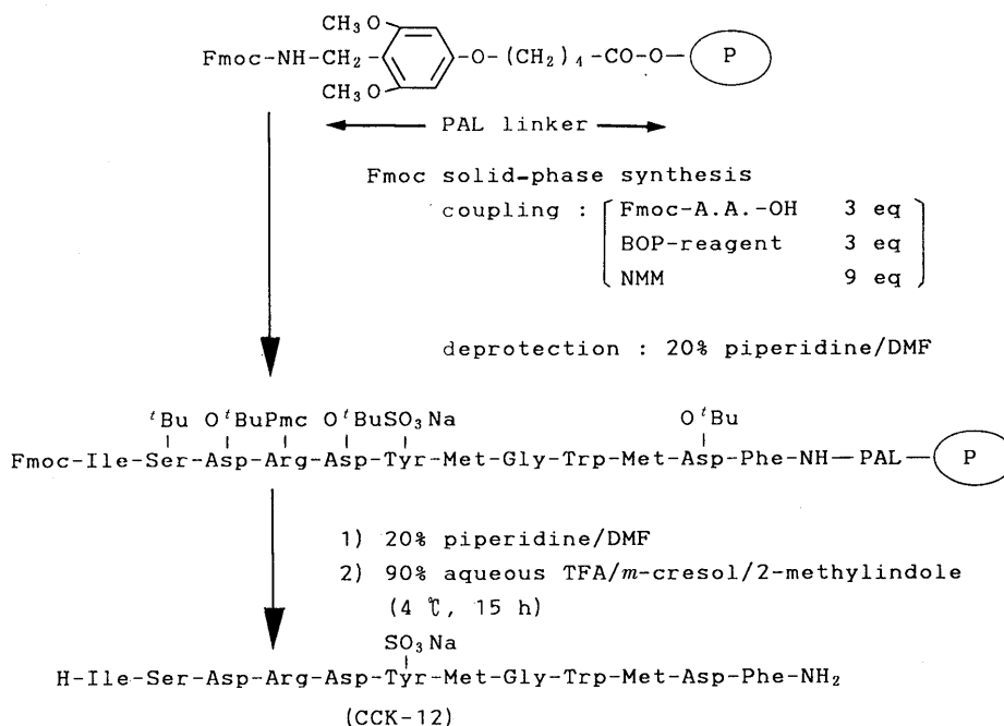
Fig. 5. Fmoc-Based Solid-Phase Synthesis of Cholecystikinin-12 (CCK-12)
