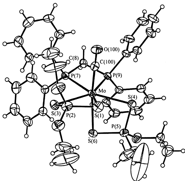
Fig. 4. An ORTEP view of [\text{Mo}(\text{CO})(\text{dppm})\{\text{S}_2\text{P}(\text{OEt})_2\}_2] ( 4a ), with thermal ellipsoids drawn at 30% probability. The atom numbering scheme of the phenyl and ethoxy groups is omitted for clarity.
