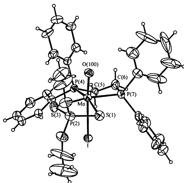
Fig. 6. An ORTEP view of [\text{Mo}(\text{O})(\text{I})(\text{dppe})\{\text{S}_2\text{P}(\text{OEt})_2\}_2] ( 7a ), with thermal ellipsoids drawn at 20% probability. The atom numbering scheme of the phenyl and ethoxy groups is omitted for clarity.
