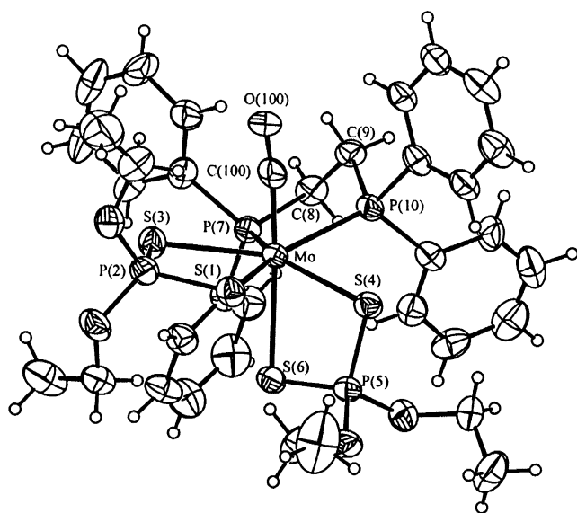
Fig. 5. An ORTEP view of [\text{Mo}(\text{CO})(\text{dppe})\{\text{S}_2\text{P}(\text{OEt})_2\}_2] ( 5a ), with thermal ellipsoids drawn at 20% probability. The atom numbering scheme of the phenyl and ethoxy groups is omitted for clarity.
