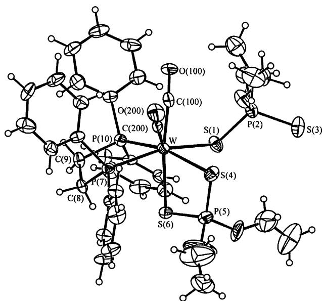
Fig. 3. An ORTEP view of [\text{W}(\text{CO})_2(\text{dppe})\{\text{S}_2\text{P}(\text{OEt})_2\}_2] ( 6b ), with thermal ellipsoids drawn at 30% probability. The atom numbering scheme of the phenyl and ethoxy groups is omitted for clarity.
