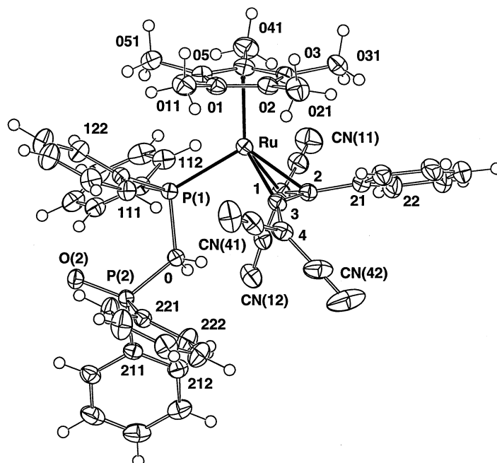
Fig. 5. Plot of a molecule of Ru\{\eta^3-C(CN)_2CPhC=C(CN)_2\}(dppmO)Cp^* ( 5 ) showing atom numbering scheme.
