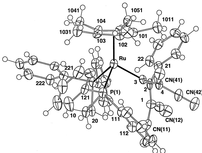
Fig. 3. Plot of a molecule of \text{Ru}\{\text{C}[\text{C}(\text{CN})_2]\text{CPh}=\text{C}(\text{CN})_2\}(\text{dppe})\text{Cp}^* ( 7 ) showing atom numbering scheme.
