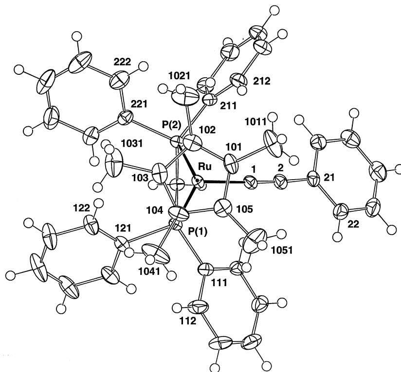
Fig. 1. Plot of a molecule of Ru(C≡CPh)(dppm)Cp* ( 1 ), showing atom numbering scheme.
