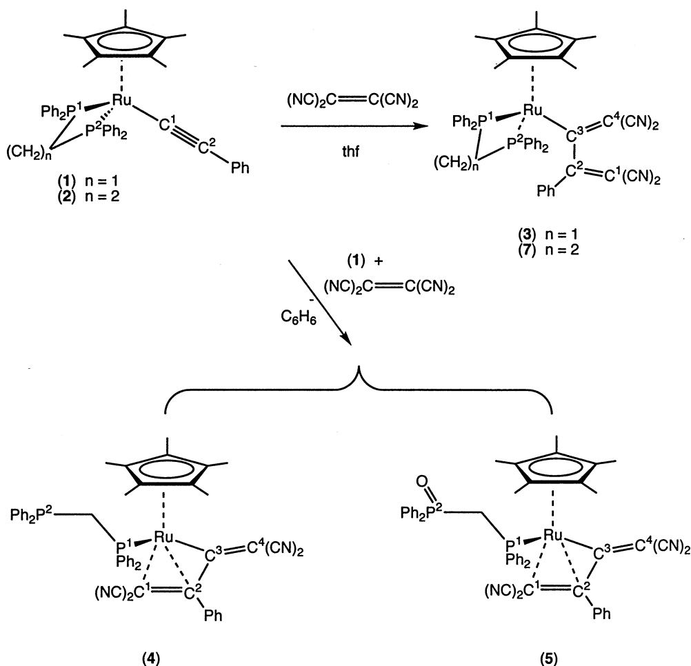
Scheme 2.
