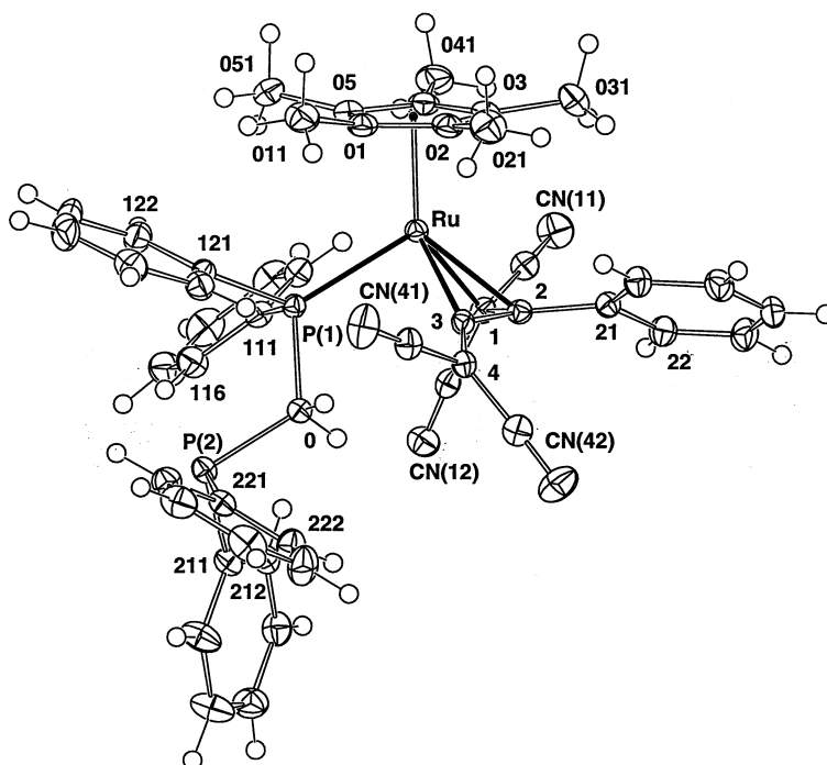
Fig. 4. Plot of a molecule of \text{Ru}\{\eta^3\text{-C}(\text{CN})_2\text{CPhC}=\text{C}(\text{CN})_2\}(\text{dppm-}P)\text{Cp}^* ( 4 ) showing atom numbering scheme.
