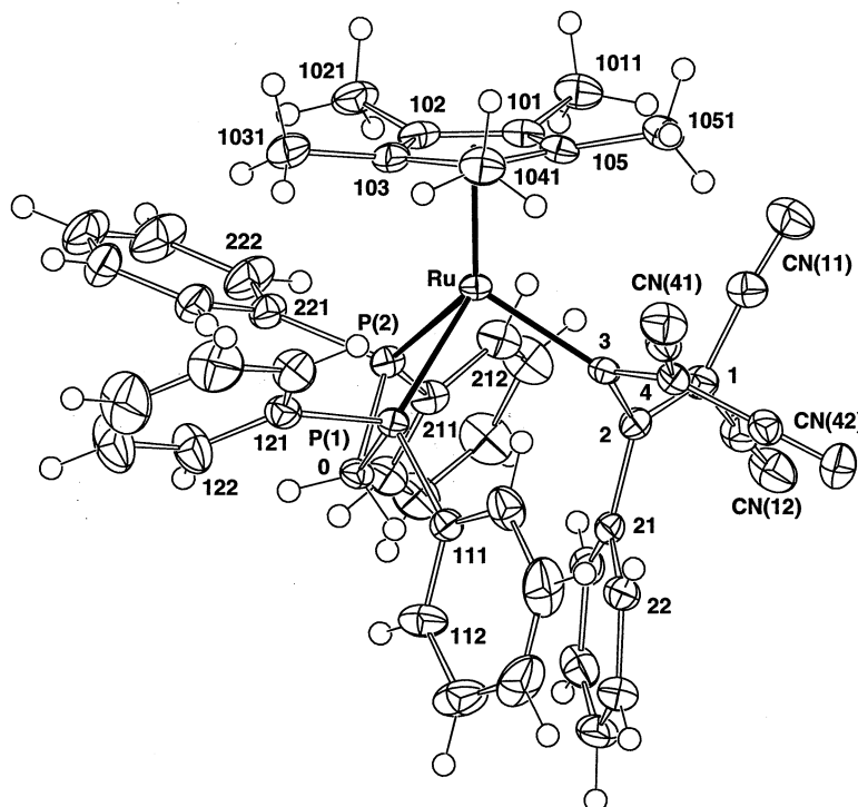
Fig. 2. Plot of a molecule of Ru{C[=C(CN) 2 ]CPh=C(CN) 2 } (dppm)Cp* ( 3 ) showing atom numbering scheme.
