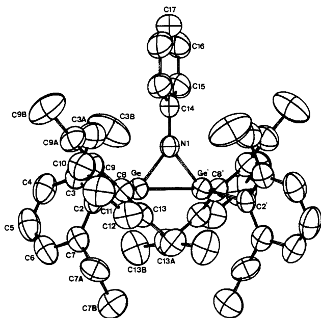
Figure 3. Molecular conformation and atomic labeling of 5 .
