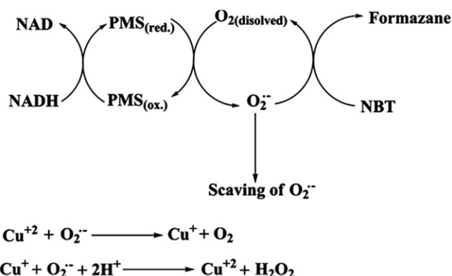
Fig. 9. Mechanism for SOD-like activity performed using the NBT/NADH/PMS system.
