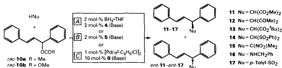
Scheme 2. Reactions of 1,3-Diphenylallyl Acetate or Methyl Carbonate with Various Nucleophiles in the Presence of the Pd Complexes 4 and 5 and of the Complex Formed from Allylpalladium Chloride and 9 , with Enantioselective Formation of the Products 11–17 . Enantiomer enrichment of product 11 by crystallizing removal of the rac -form.
