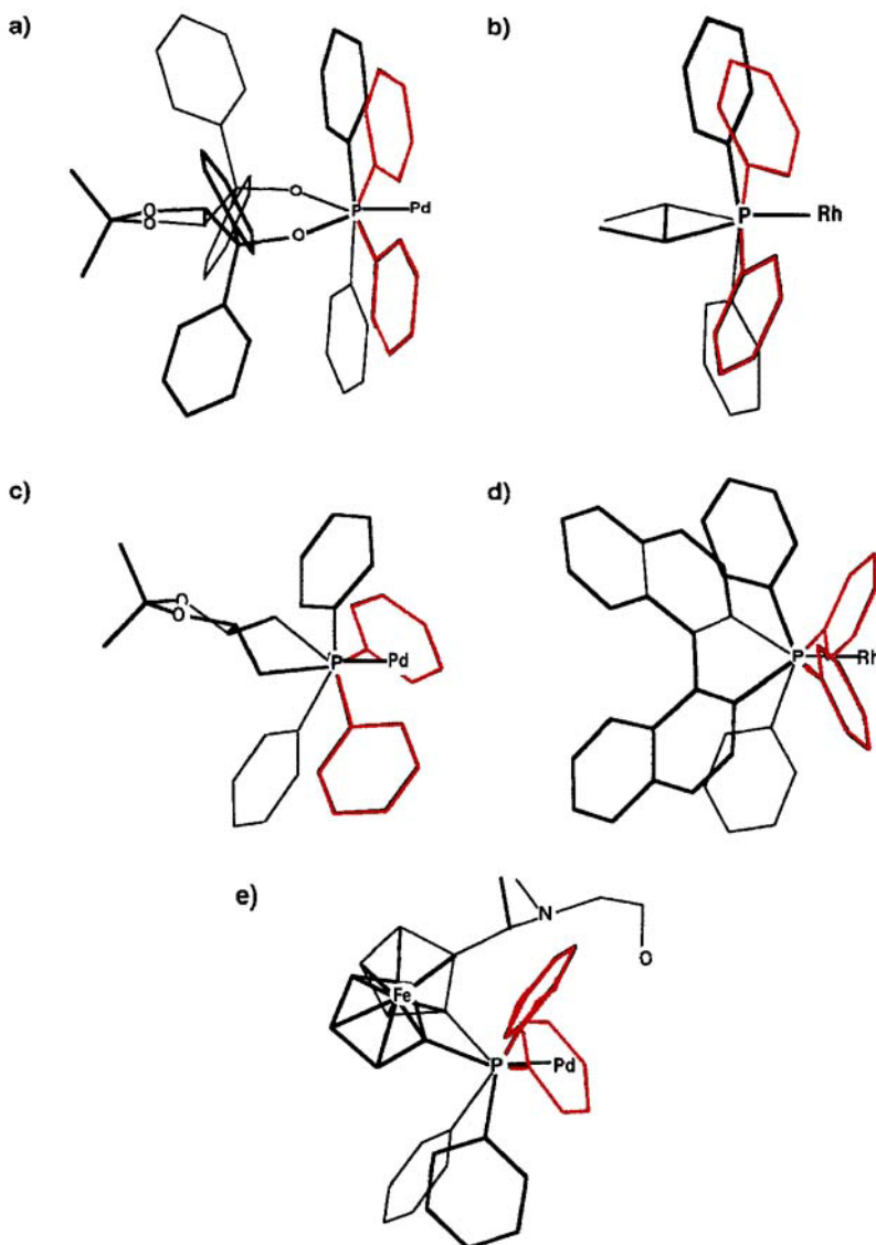
Fig. 2. View along the \text{P} \cdots \text{P} vector of some transition-metal complexes of bidentate \text{Ph}_2\text{P} ligands. a) ( R,R )-taddop, b) ( S,S )-chiraphos (CUYYAW), c) ( S,S )-diop (BICLOO), d) ( P )-binap (BNAPRH), and e) ( R )-( S )-bppf (JARSIE). The quasi-equatorial Ph groups are depicted in red (bold print of Ph in front). Note that the equatorial Ph groups are closer to the metal center than the axial ones. The CSD codes are given in parentheses.
