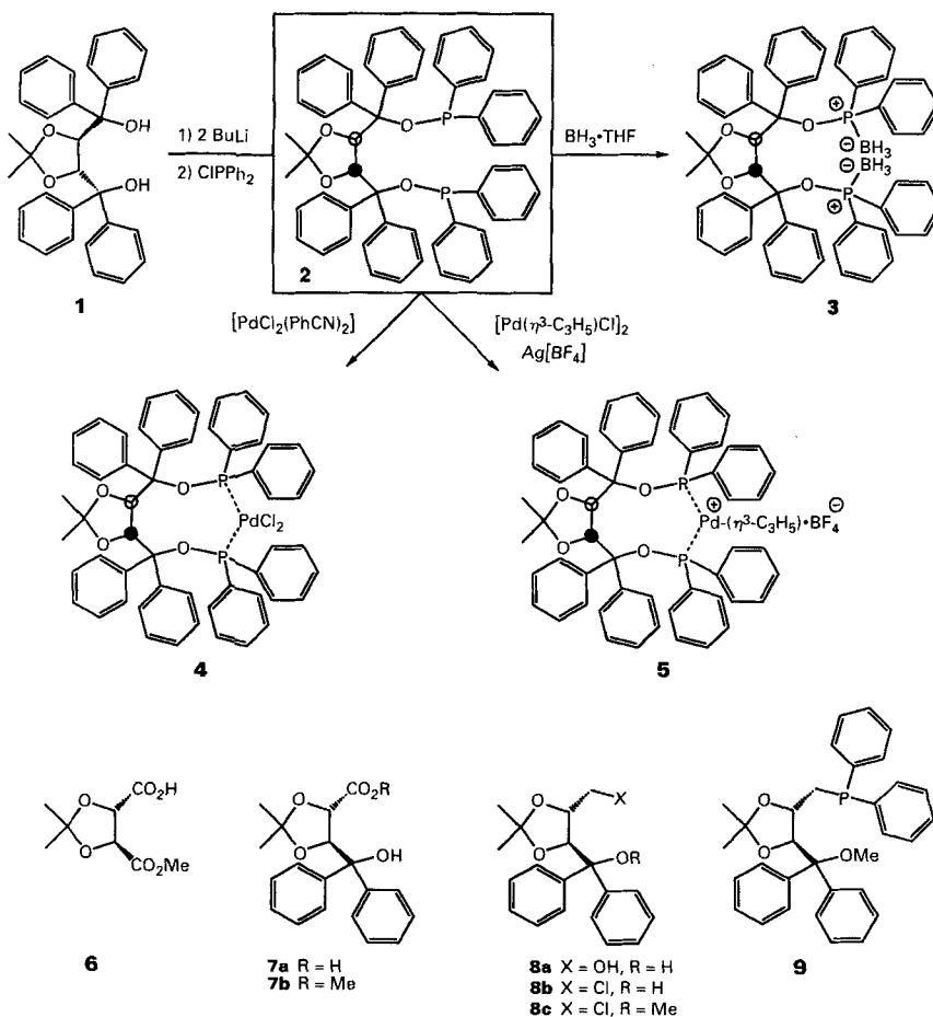
Scheme 1. Preparation of the taddop Ligand 2 and of the Corresponding Pd Complexes 4 and 5 . The unsymmetric 9 and intermediates 6–8 in its preparation.
