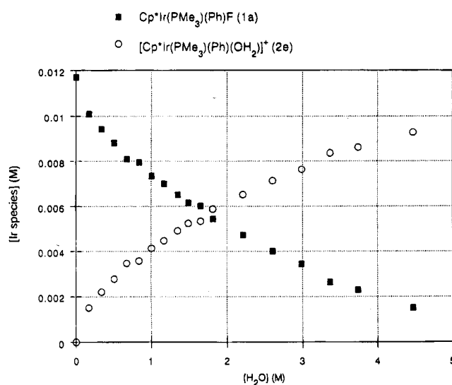
Figure 1. Titration of \text{H}_2\text{O} against \text{Cp}^*\text{Ir}(\text{PMe}_3)(\text{Ph})\text{F} ( 1c ) in \text{THF-d}_8 .
