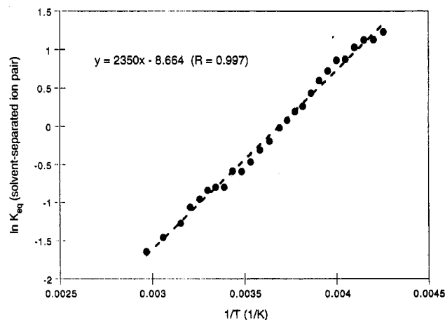
Figure 2. Plot of \ln K_{\text{eq}} (for a solvent-separated ion pair) against 1/T .
