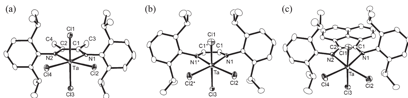
Figure 4. Molecular structures of ( \alpha -diimine) \text{TaCl}_4 ((a) 8a, (b) 8b, and (c) 8c) with 30% thermal ellipsoids. All hydrogen atoms are omitted for clarity.
