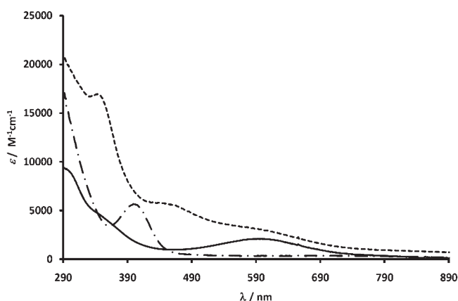
Figure 7. UV–vis spectra of 8b (—), 9b (---) and 10b (····) in \text{CH}_2\text{Cl}_2 at 25 °C.
