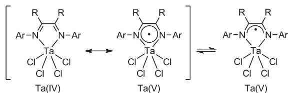
Chart 2. Coordination Mode of \alpha -Diimine Ligands for (\alpha\text{-Diimine})\text{TaCl}_4
