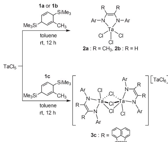
Scheme 1. Preparation of Tantalum Complexes with Dianionic \alpha -Diimine Ligands Using MBTCD as a Reductant
