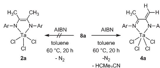
Scheme 7. Reaction of 8a with AIBN-Derived Carbon Radical
