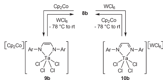
Scheme 5. Chemical Oxidation and Reduction Reactions of 8b
