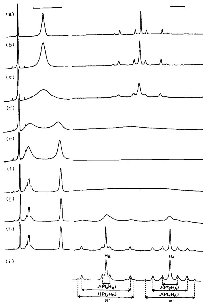
Fig. 8. The ^1\text{H} NMR (400 MHz) spectra of [\text{Pt}_2\text{H}_2(\mu\text{-Cl})(\mu\text{-dppm})_2]^+ in \text{CD}_2\text{Cl}_2 at (a) +23 , (b) +5 , (c) -5 , (d) -15 , (e) -25 , (f) -35 , (g) -45 , and (h) -55^\circ\text{C} . The bars represent 400 Hz. (i) represents the computer simulation of the hydride region of (h).
