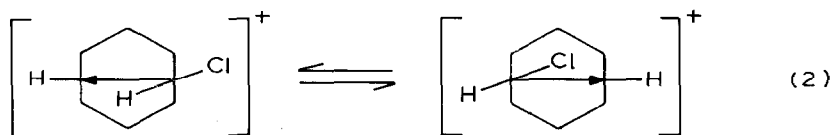
Fig. 10. The ^{195}\text{Pt}\{^1\text{H}\} (19.16 MHz) NMR spectra of [\text{Pt}_2\text{H}_2(\mu\text{-Cl})(\mu\text{-dppm})_2][\text{PF}_6] in \text{CD}_2\text{Cl}_2 at (a) +30, (b) -2, (c) -25, (d) -58, and (e) -70°C. The bar represents 3000 Hz. (f) represents the computer simulation of the hydride region of (e).
