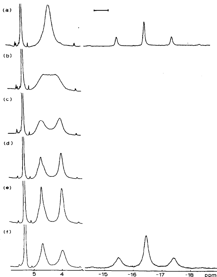
Fig. 6. The ^1\text{H} NMR (400 MHz) spectra of [\text{Pt}_2\text{Cl}_2(\mu\text{-H})(\mu\text{-dppm})_2]^+ in \text{CD}_2\text{Cl}_2 at (a) +23 , (b) +10 , (c) 0 , (d) -10 , (e) -30 , and (f) -50^\circ\text{C} . The bar represents 200 Hz.
