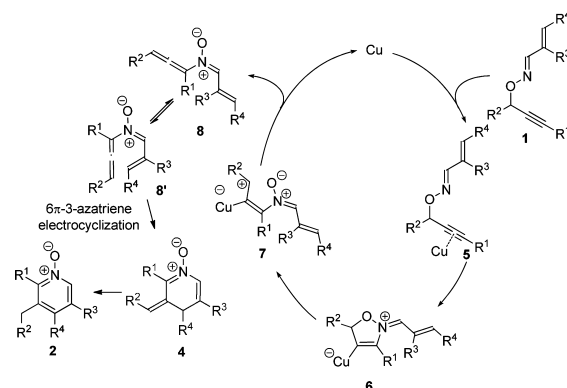
Scheme 1. Plausible Mechanism
