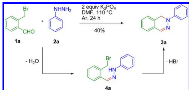
Scheme 1. Initial Experiment for the Synthesis of 2-Substituted 1,2-Dihydrophthalazines
