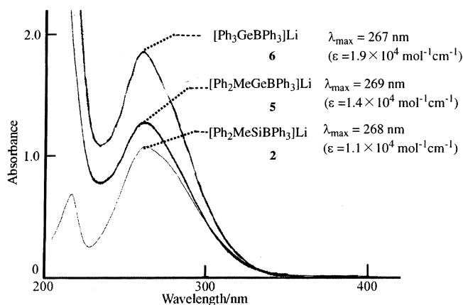
Figure 5. Absorption spectra of phenyl-substituted silyl- and germylborates in THF at 23^\circ\text{C} . Optical path length is 1 cm.
