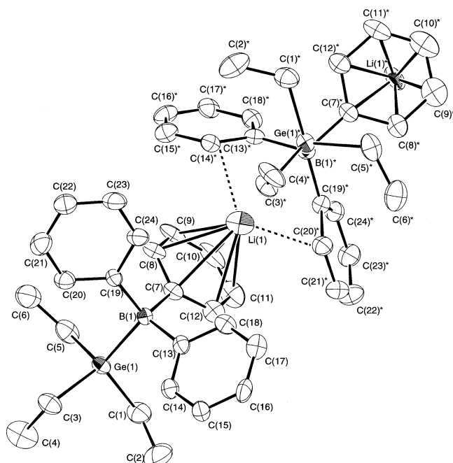
Figure 2. Molecular structure of 7 at the 50% probability level. Hydrogen atoms are omitted for clarity.
