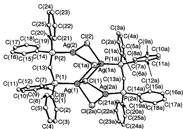
Fig. 2 Molecular structure of [\text{Ag}_4\text{Cl}_4(\text{dppm})_2] \cdot 3
