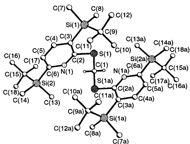
Fig. 3 Molecular structure of R 2 SCH 2 SR 2
