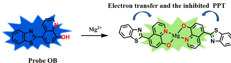
Fig. 1. Our fluorescent probe for \text{Mg}^{2+} ion.
