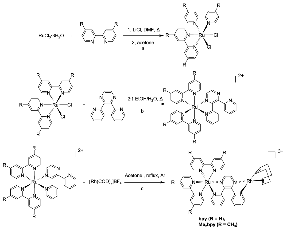
Figure 2. Synthetic scheme of [(\text{bpy})_2\text{Ru}(\text{dpp})\text{Rh}^{\text{I}}(\text{COD})](\text{PF}_6)_3 and [(\text{Me}_2\text{bpy})_2\text{Ru}(\text{dpp})\text{Rh}^{\text{I}}(\text{COD})](\text{PF}_6)_2(\text{BF}_4) . a Adapted from ref 44. b Adapted from ref 43. c Adapted from ref 41.
