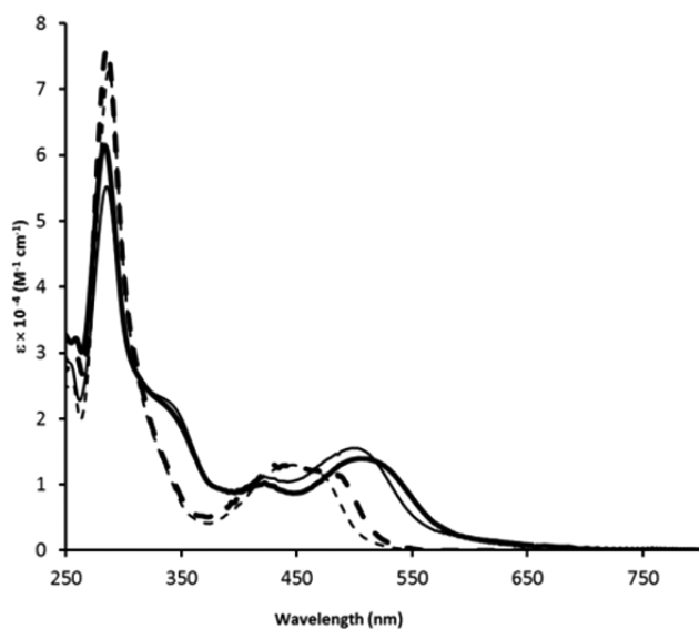
Figure 8. Electronic absorption spectra for the [(bpy)_2Ru(dpp)Rh^I(COD)](PF_6)_3 (—), [(bpy)_2Ru(dpp)](PF_6)_2 (---), [(Me_2bpy)_2Ru(dpp)Rh^I(COD)](PF_6)_2(BF_4) (— · —), and [(Me_2bpy)_2Ru(dpp)](PF_6)_2 (····) measured in deoxygenated dry CH_2Cl_2 at room temperature (bpy = 2,2'-bipyridine, Me_2bpy = 4,4'-dimethyl-2,2'-bipyridine, dpp = 2,3-bis(2-pyridyl)pyrazine, and COD = 1,5-cyclooctadiene).
