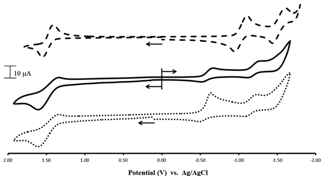
Figure 7. Cyclic voltammograms of [(bpy)_2Ru(dpp)](PF_6)_2 (top, dashed line) and [(bpy)_2Ru(dpp)Rh^I(COD)](PF_6)_3 (middle, solid line, and bottom dotted line) in 0.1 M ^tBu_4NPF_6 in CH_2Cl_2 solution using a platinum disk working electrode, platinum wire auxiliary electrode, and silver wire as reference electrode ( FeCp_2^{+/0} = 0.46 V vs Ag/AgCl). Scan direction is indicated by an arrow (bpy = 2,2'-bipyridine, dpp = 2,3-bis(2-pyridyl)pyrazine, and COD = 1,5-cyclooctadiene).
